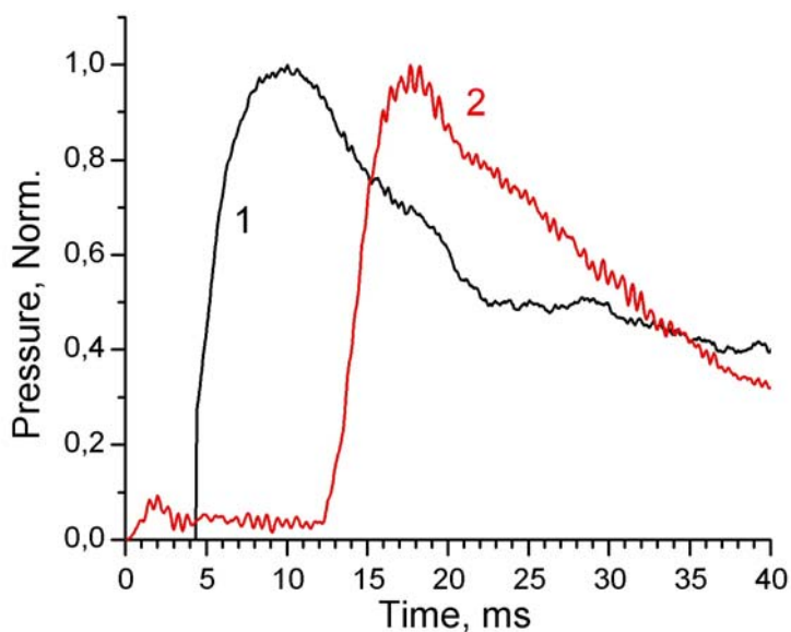
Fig. 29. Time dependences of pressure in the tube (1) and in the nuzzle prechamber (2).
