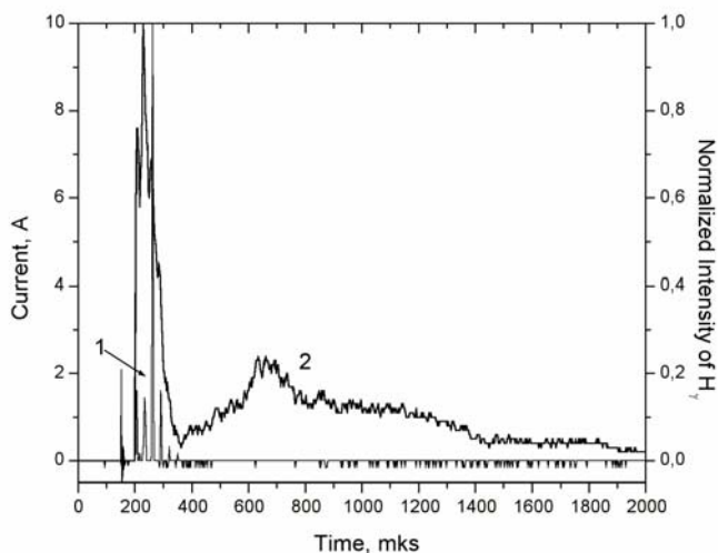
Fig. 13. Intensity of atomic hydrogen line H_{\gamma} , normalized for maximum (2), and synchronic – the amplitude of the collector current (the current passing through the mixture and captured in the collector) (1). Stoichiometry mixture.
