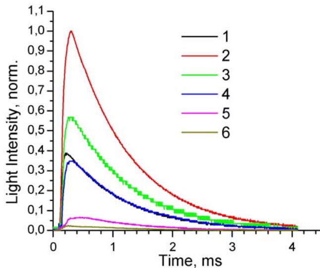
Fig.40. Time dependencies of CH irradiation band (about 430nm) intensities normalized by maximum (for all diagrams) value.
