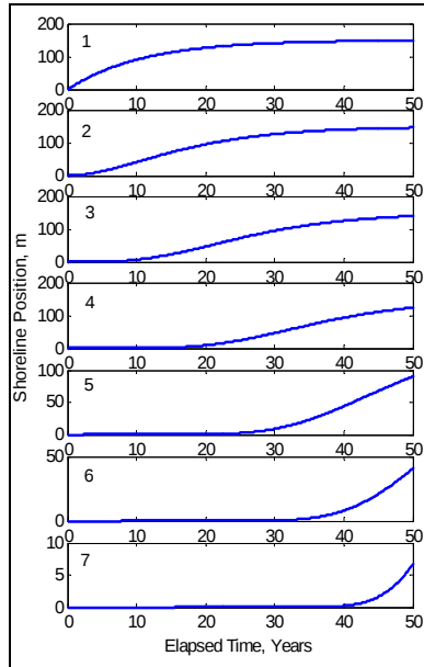
Figure 3. Equi-length groins (groin compartments 1-7, top - bottom).
