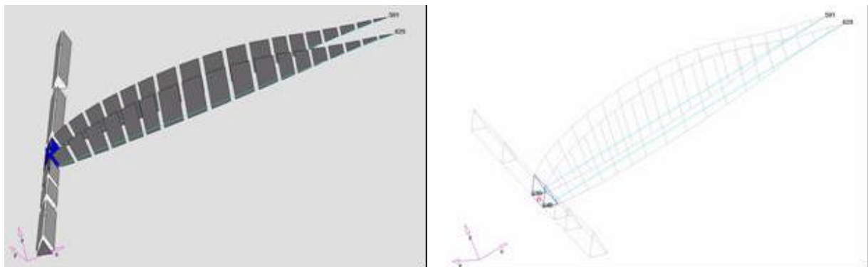
Figure 4. Stiffened structural elements, “leading edge” elements t=40\text{mm} , ribs elements t=5\text{mm}
