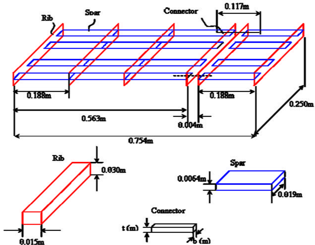
Figure 6. Dimensions of Model With / Without Device
