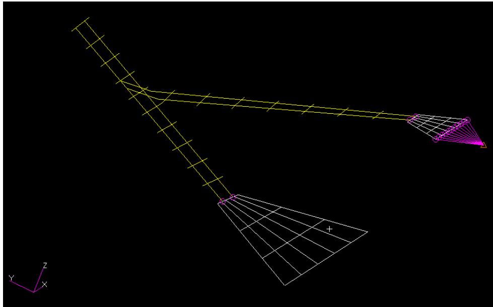
Figure 25. Two Spar Wing Tunnel Model Internal Structure FE Mesh
