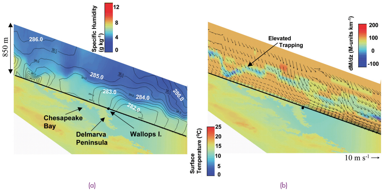
FIGURE 5 COAMPS™ forecast valid 10 a.m. LT April 29, 2000 of surface temperature (°C) in the foreground. Cross sections of (a) color shaded specific humidity and potential temperature contours (K), and (b) wind vectors in the plane of the cross section and color shaded dM/dz . Blue regions indicate EM trapping, while dark red is subrefractive.
