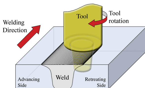
FIGURE 8 Schematic of the friction stir welding process.
