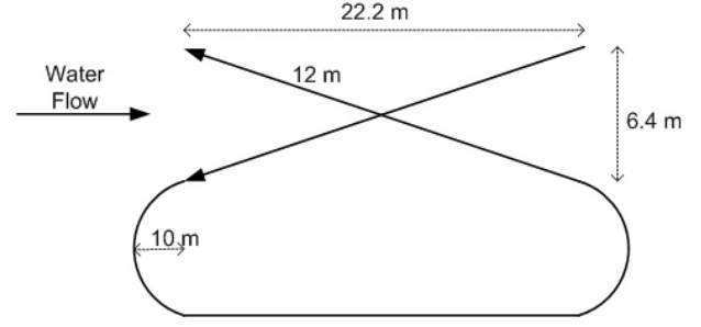
Figure 3: Bowtie maneuver
