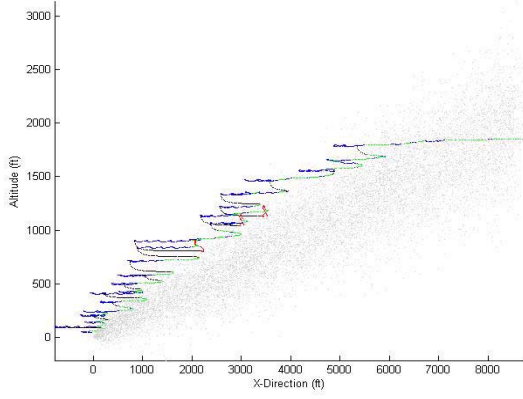
Figure 17: Vertical plane of a successful run - plume B, sensor A, \zeta = 180 s and \Delta T_{ct} = 10 s
