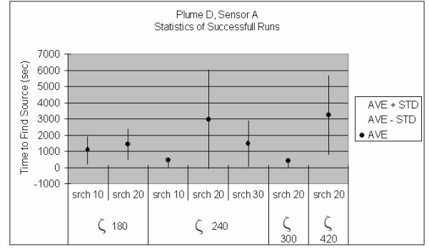
Figure 19: Plume D, Sensor A - Statistics for the time to source for successful Monte Carlo runs
