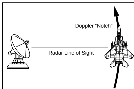
Figure 3. Doppler-Notch Diagram. The target aircraft must fly a curved line to maintain a constant distance from the radar and remain in the zero-Doppler region.
