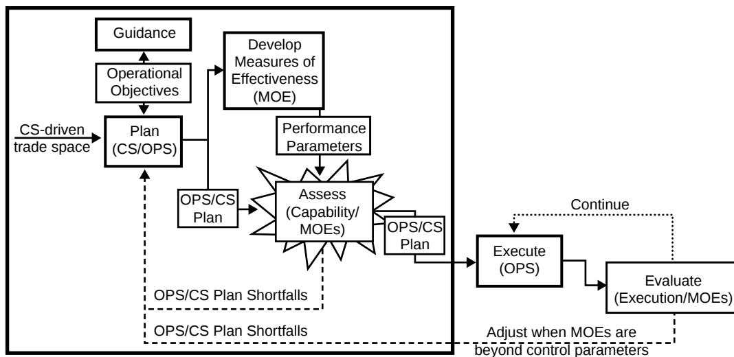
Figure 1. CS C2 Concept Process
