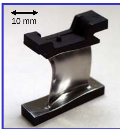
Figure 3: Single MIM Compressor vane
