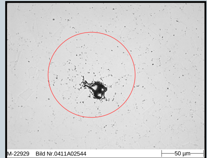
Micrograph picture of a carbide agglomeration
