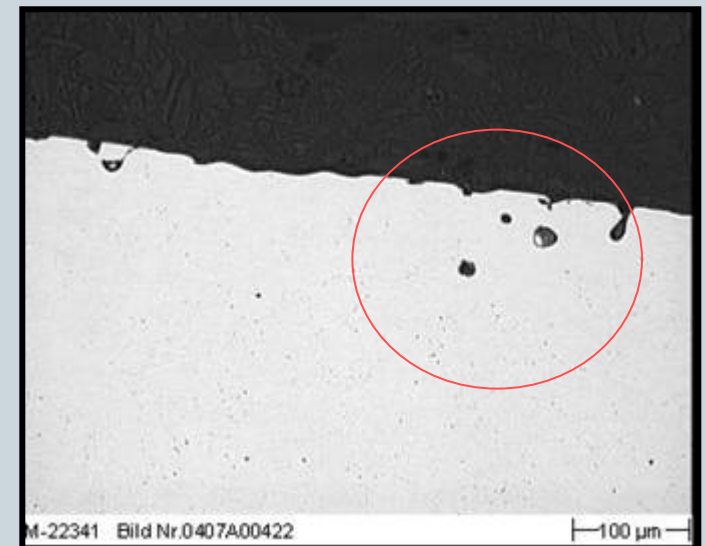
Microscope picture of porosity close to the surface
