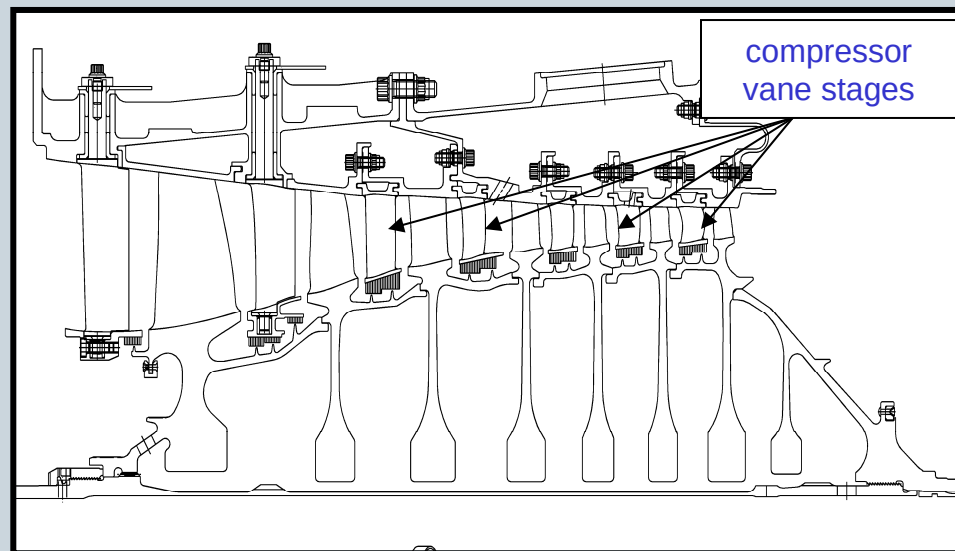
High Pressure Compressor (Schematic)
