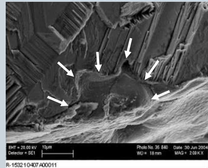
Fatigue crack in MIM material
