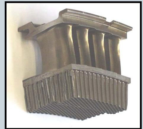
Four MIM vanes brazed together for a vane clusters
