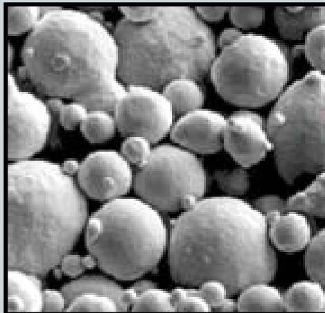
Pure Nickel alloy powder micrograph
