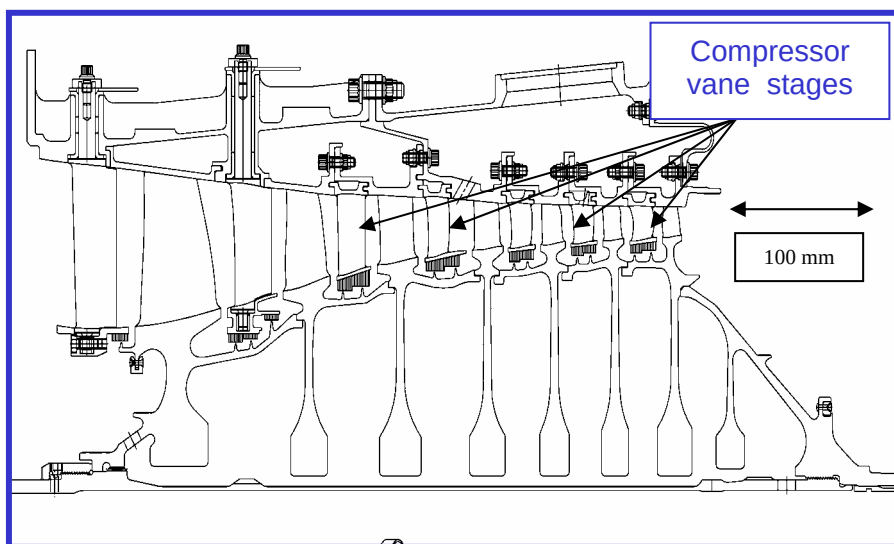
Figure 2: High-pressure compressor (schematic)
