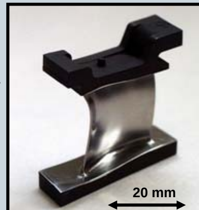
Prototype MIM compressor vane
