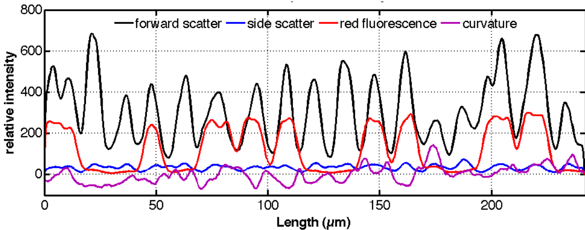
Figure 7. A pulse profile from the same culture of Chaetoceros compressus var. hirtisetus several days later, after it had reached senescence. Note the many dead cells, which contain no chlorophyll.
