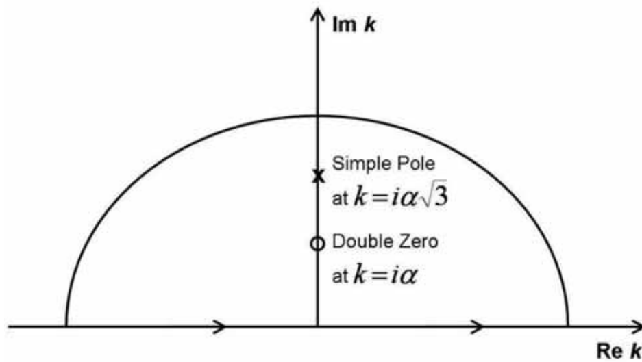
Figure 1. Poles and zeros of \mathcal{L}^+(k) in the upper half plane for the Saito potential. Poles are indicated by x , zeros by o . There are no poles or zeros of \mathcal{L}^+(k) on the real axis.
