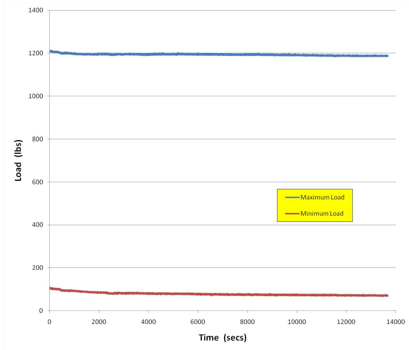
Figure 4. Cyclic Load vs. Time, Case #3a
