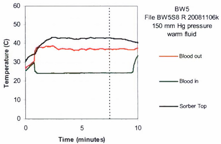
Figure 7. Performance of three prototypes with 150 mm Hg infuser pressure and warm fluid.
