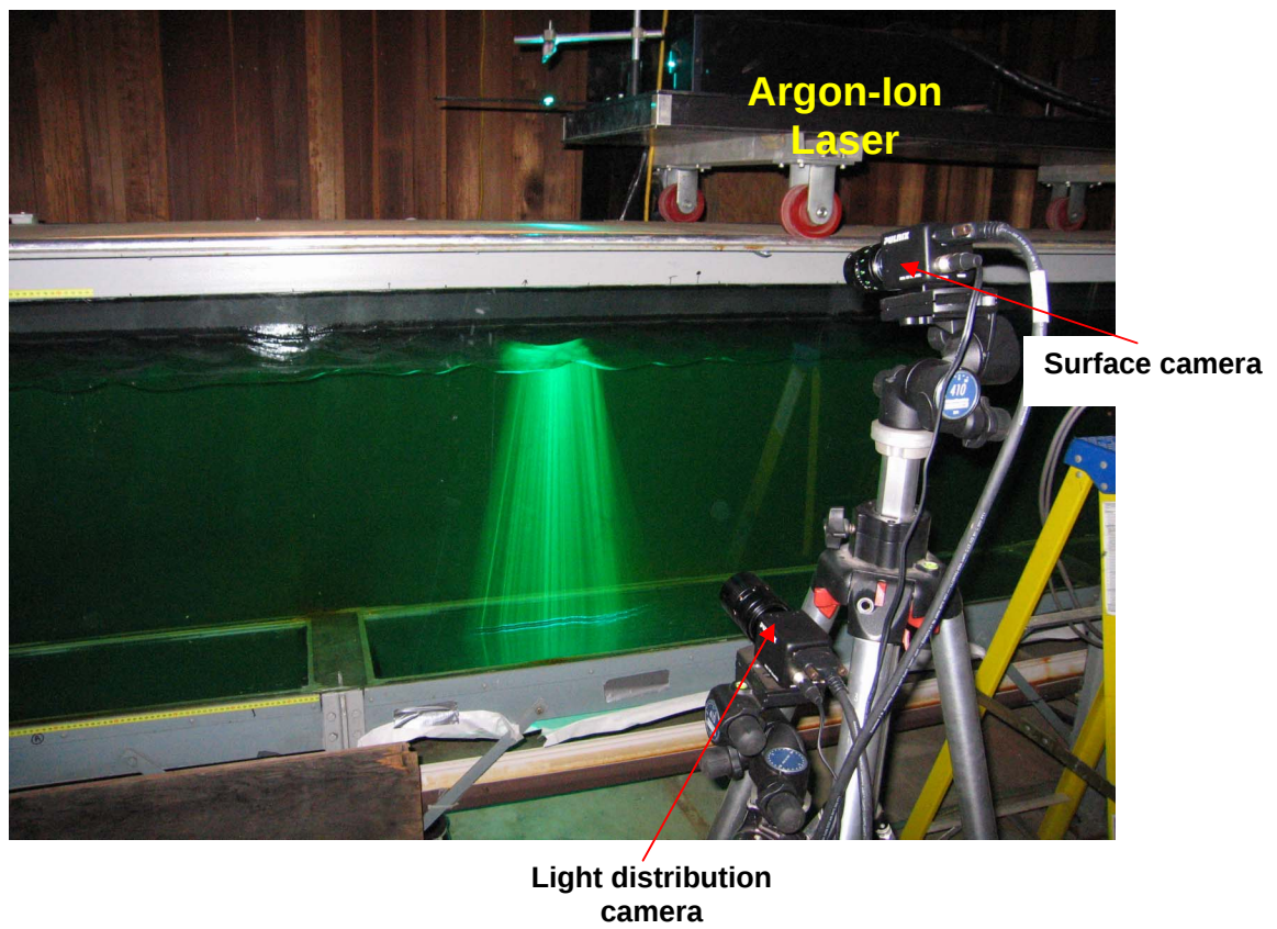
Figure 2: Laboratory Setup.
