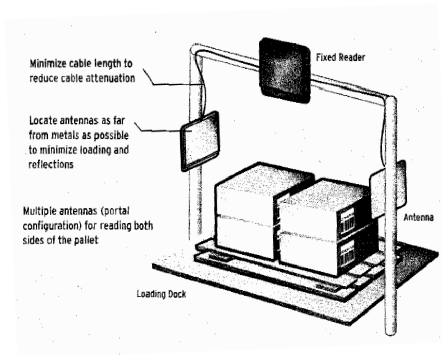
Figure 6. Archway Portal Reader[1].
