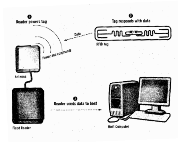
Figure 3. Tag-Read-Host Communication[1].
