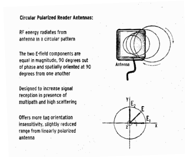
Figure 9. Circular Polarized Antenna[1].
