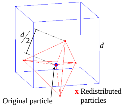
Figure 4. Schematic of vorticity redistribution scheme.
