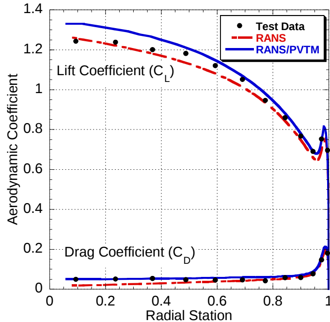
Figure 8. Lift and drag coefficients along wing span derived from surface pressures.
