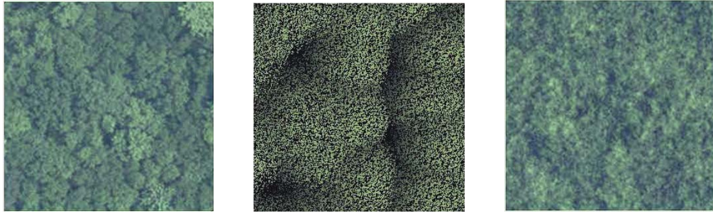
Figure 8: Comparison of our synthesized image and DIRSIG image.
