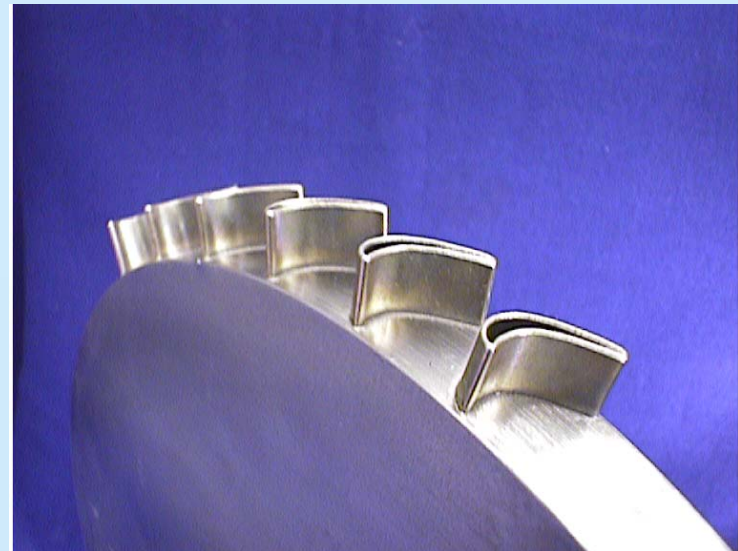
Building airfoils on turbine disc to form a "blisk".
