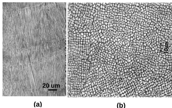
Figure 3: Microstructure of LC IN-625 alloy (a) vertical cross-sectional view, and (b) horizontal cross-sectional view.
