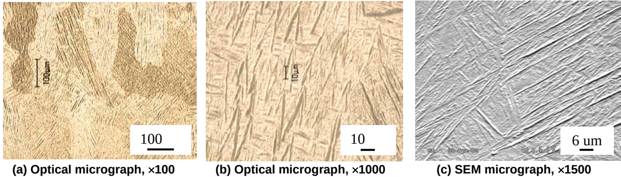
Figure 6: Microstructure of LC Ti-6Al-4V.
