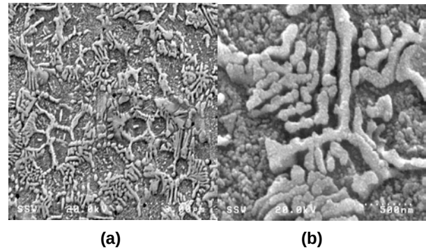
Figure 8: Microstructure of LC CPM-9V by high resolution SEM, (a) \times 6,500 , and (b) \times 40,000 .
