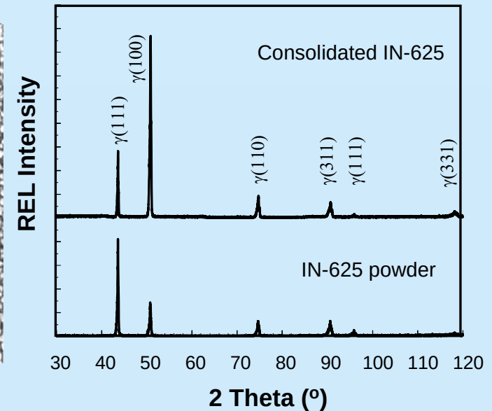
Comparison of XRD pattern of laser consolidated IN625 with the powder.
