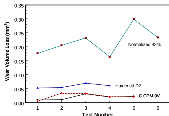
Figure 9: Pin-on-disk wear test results (disk volume loss).
