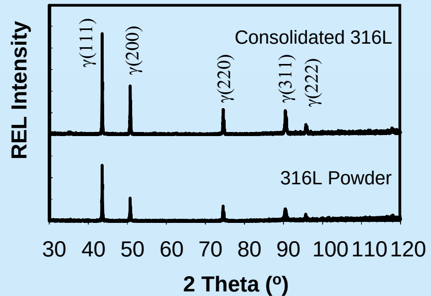
Comparison of XRD patterns of LC 316 SS and the powder used.
