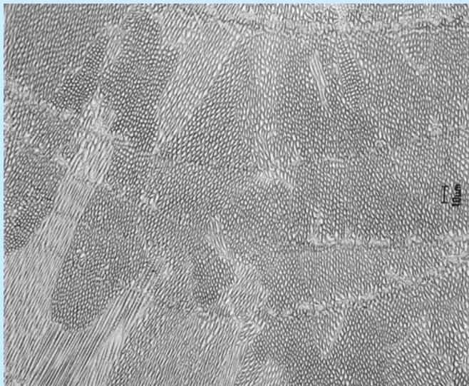
Microstructure of LC 316 stainless steel.
