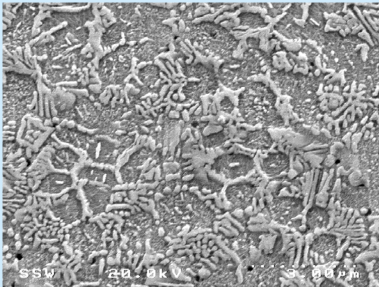
Microstructure, x 6,500
