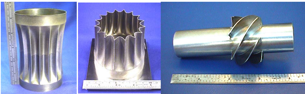
Figure 12: As-consolidated IN-625 alloy fins on a stainless steel
