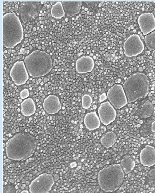
Cast IN-738, x15,000
