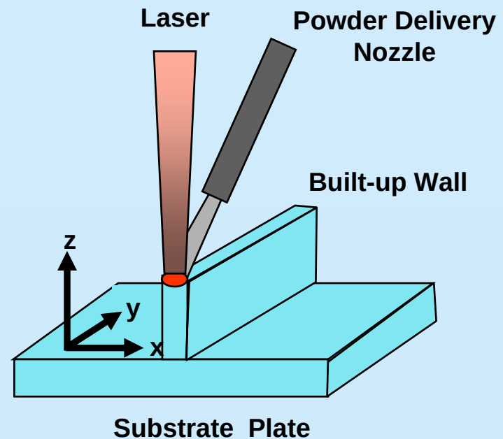
Laser Consolidation Process
