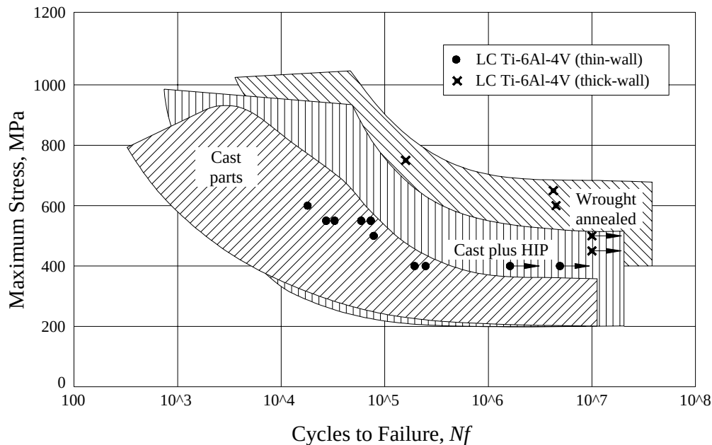
Figure 7: Fatigue data of laser consolidated Ti-6Al-4V compared with cast and wrought/anneal Ti-6Al-4V ( R=+0.1 ) [16].
