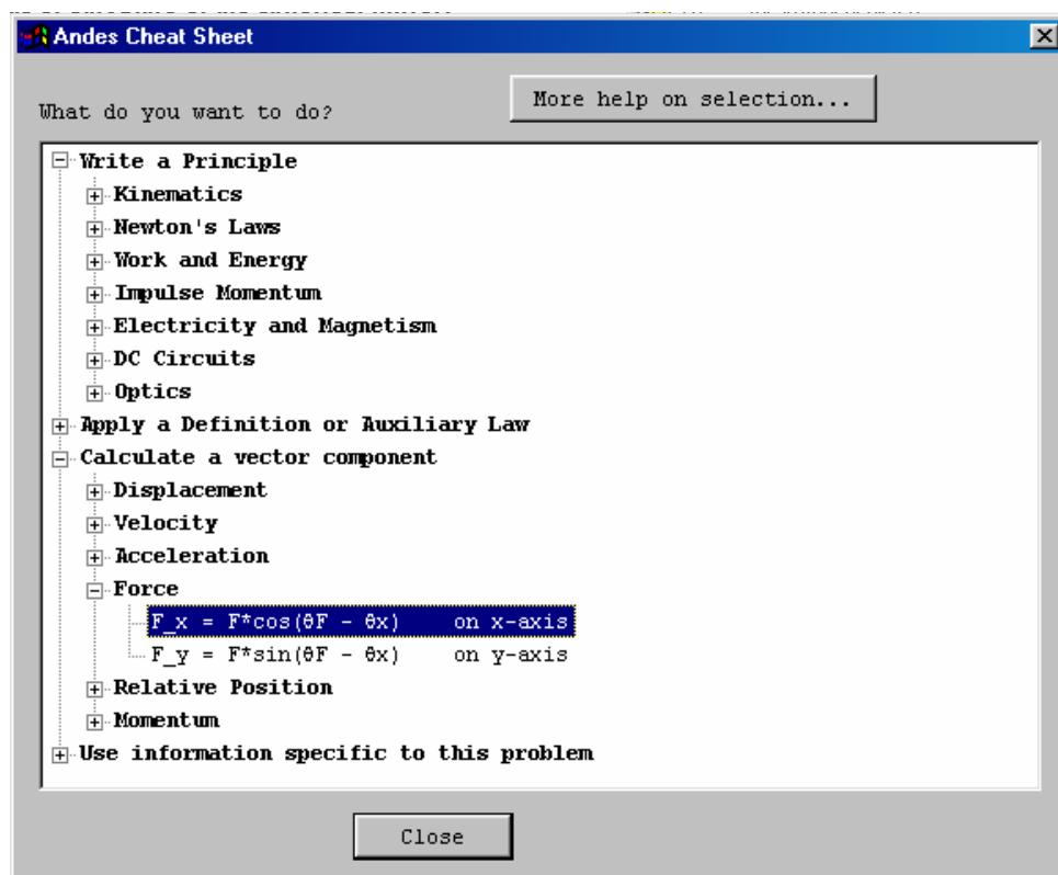
Figure 3: The Cheat Sheet is an index to unintelligent help
