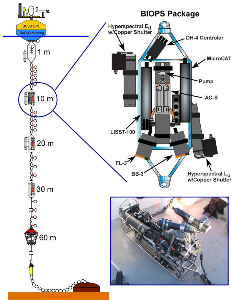
Figure 2. The RaDyO Mooring
