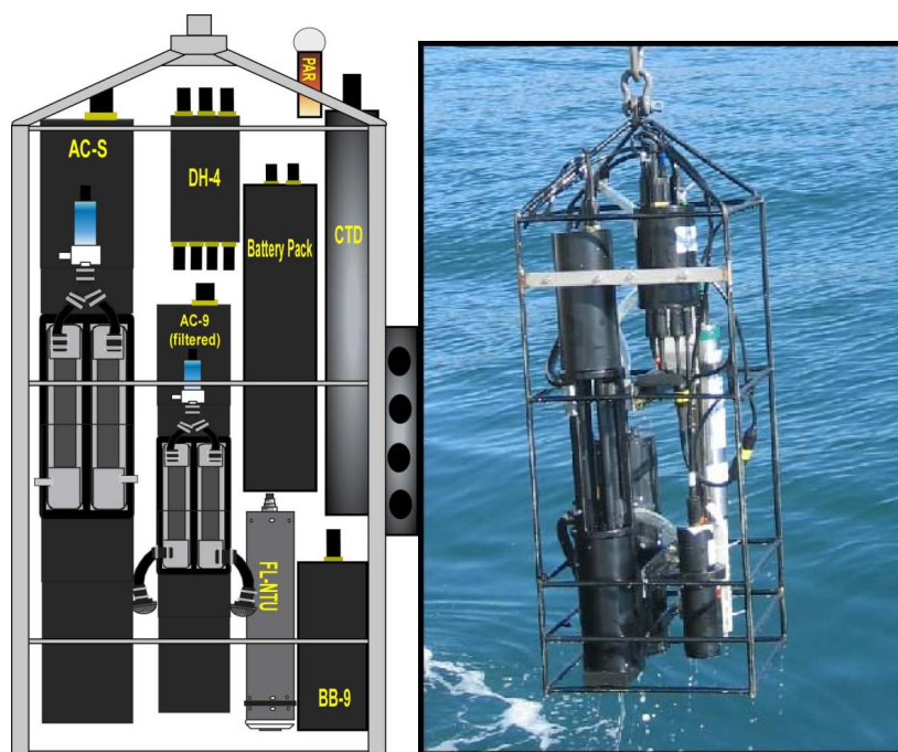
Figure 1. The Optical Profiler
