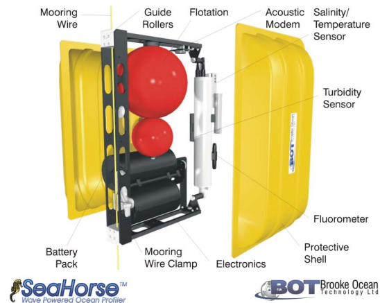
Figure 1. Schematic of the interior of the SeaHorse. Figure provided by Brooke Ocean Technology.
