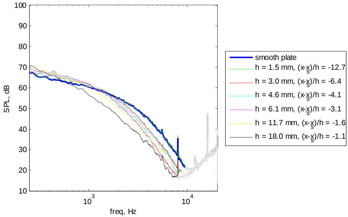
Figure 3.26. Wall Pressure Spectra at (x_s - x) / \delta = 0.92 for all Step Heights at U_j = 30 m/s
