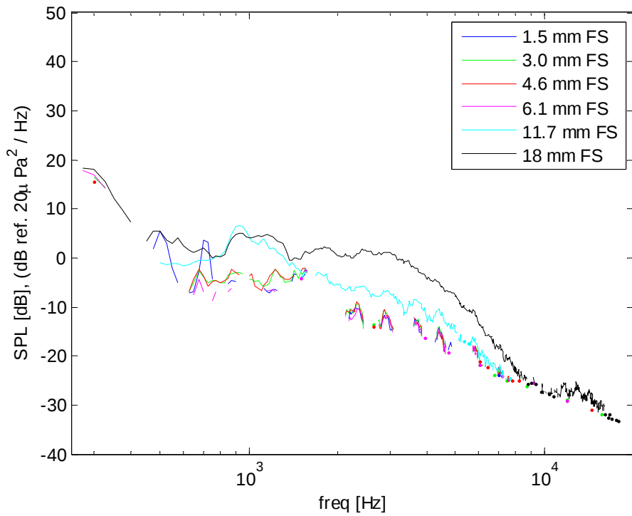
Figure 3.61 a-d. Far Field Acoustics from Narrow Asymmetric Gaps at U_j = 30 m/s at the considered Observation Angles;
