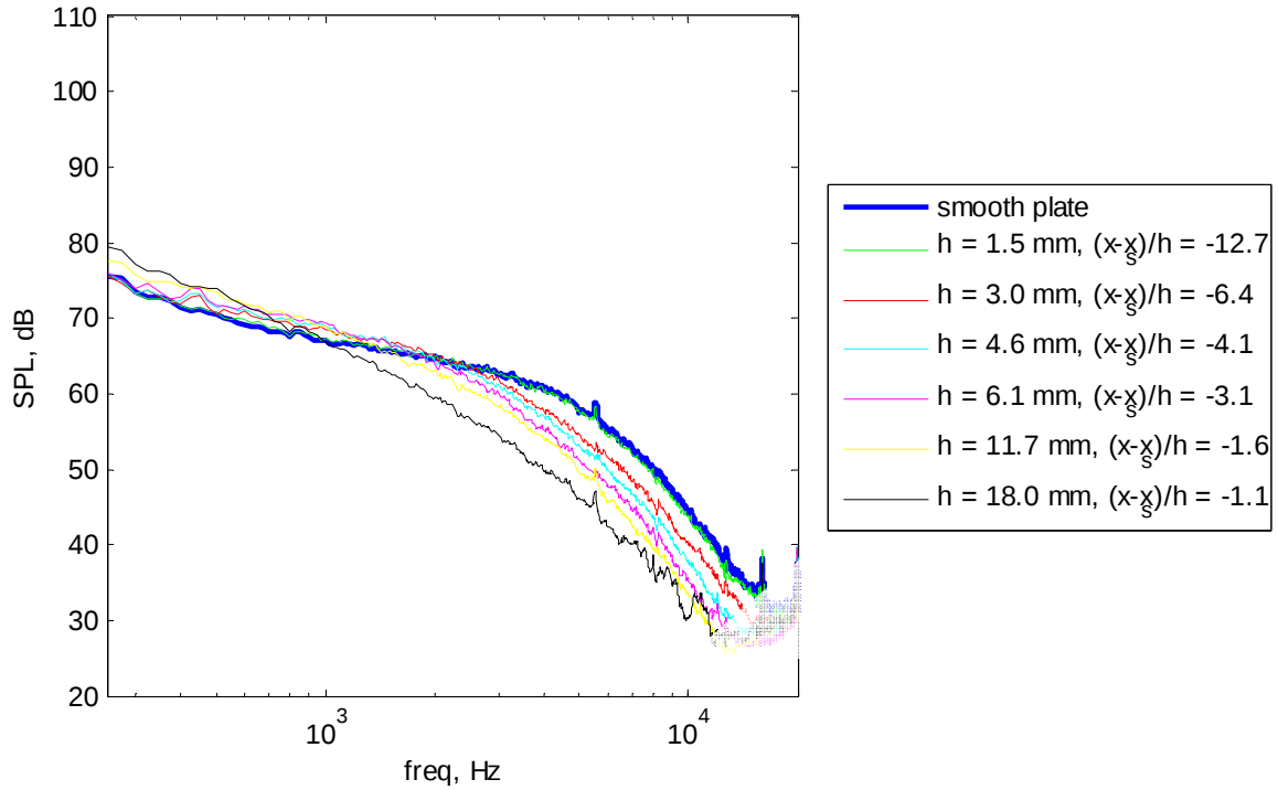
Figure 3.25. Wall Pressure Spectra at (x_s - x) / \delta = 1.01 for all Step Heights at U_j = 45 \text{ m/s}
