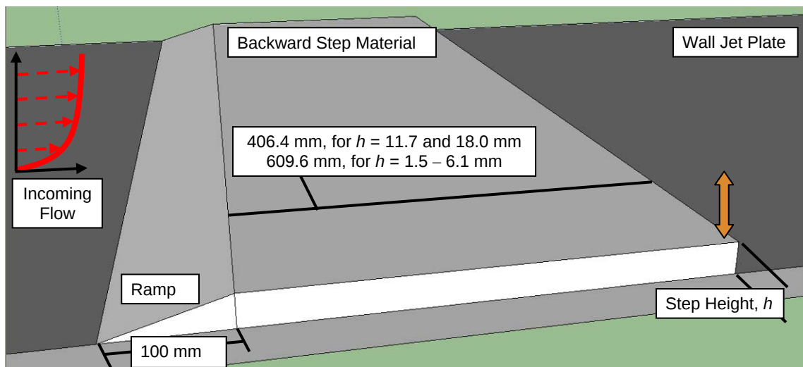
Figure 2.6. Backward Step Schematic
