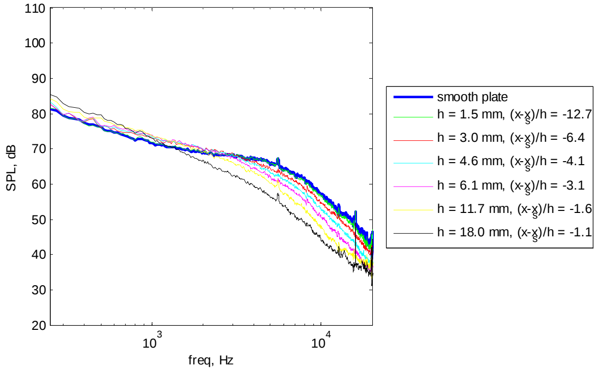
Figure 3.24. Wall Pressure Spectra at (x_s - x) / \delta = 1.07 for all Step Heights at U_j = 60 \text{ m/s}
