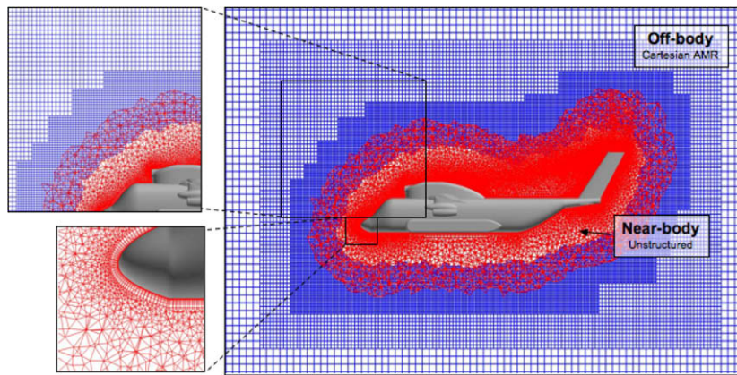
Fig. 2. Overset near/off-body gridding. Unstructured or curvilinear grids to capture geometric features and boundary layer near-body surface, adaptive block-structured Cartesian grids to capture far-field flow features.
