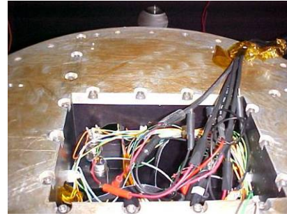
Figure 41. External Power and Data Acquisition Lines for Pressure Testing
