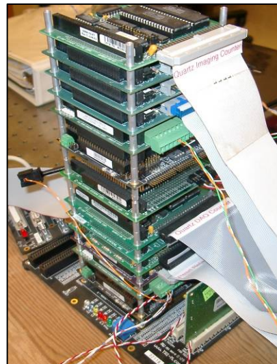
Moody's [6] two computer stack with 14 total PC-104 boards
