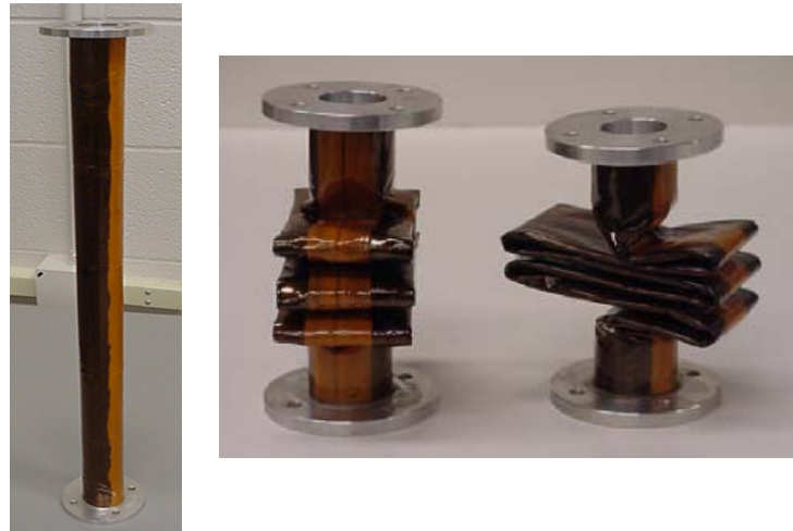
Figure 3. Rigidizable Inflatable Sub-Tg Tubes (20" long deployed) [14]
