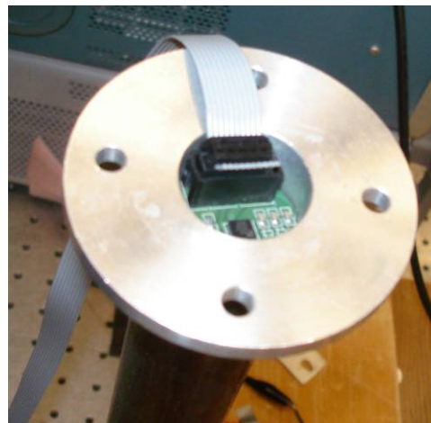
Figure 6. Lightweight Accelerometer (Kionics KXPA-4 shaped to fit into the end cap of each tube) NOTE: Shown without staking compound
