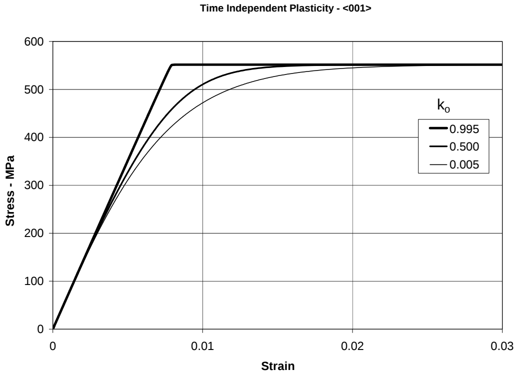
Figure 1. Typical stress-strain curves obtained with rate-independent model with different values of parameter k_0 .
