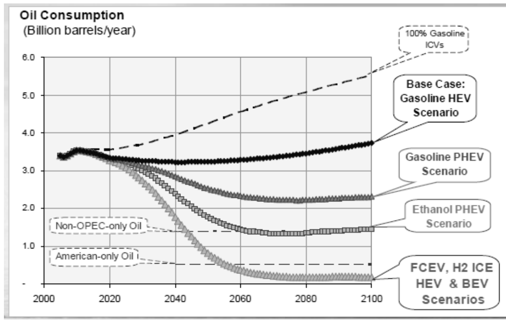
Figure 2: Impact of alternative fuel vehicles on U.S. oil consumption. 58
