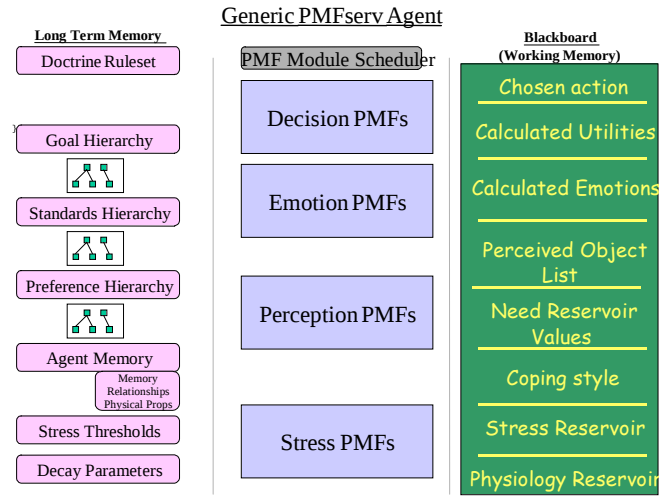
Figure 5: PMFserv Overview
