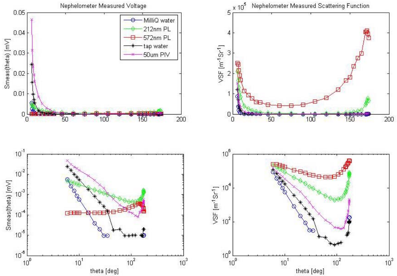
Figure 2: The nephelometer VSF particle measurements
