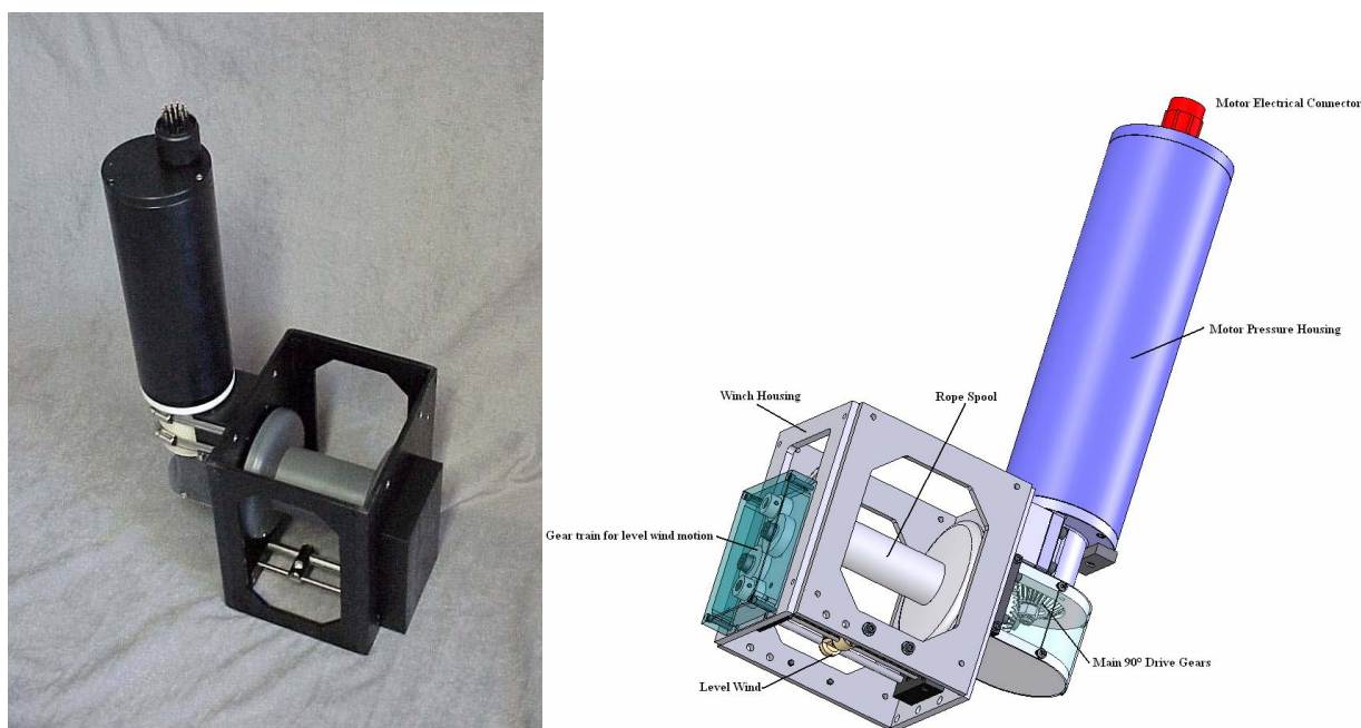
Figure 3. Picture and drawing of the winch system used on the AMP platform. Note the right angle worm gear drive, level wind and gearing, rope and rope spool. The winch drum is capable of holding 250 m of 0.07” Plasma® rope. The integral level wind ensures that the rope pays in and out in a predictable manner. To reduce wear on the winch rope, the level wind traveller and other fairleads are equipped with highly polished ceramic eyelets. A scalable gear box has also been designed to accommodate a broad range of profiling speeds.
