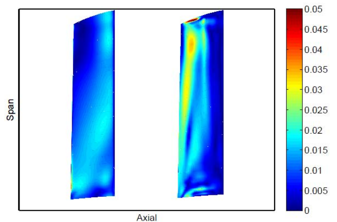
Figure 15. Unsteady pressure magnitudes normalized by stage-inlet to total pressure at the fundamental upstream vane-passing frequency (L: Pressure side, R: Suction side).
