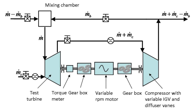
Figure 5. Schematic of the Notre Dame Turbine Facility
