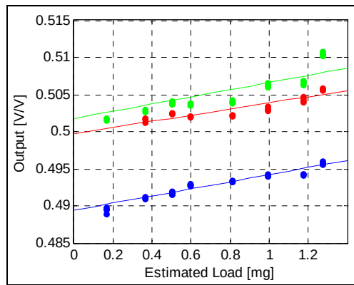
Figure 6. Calibration curves of external beam loading.
