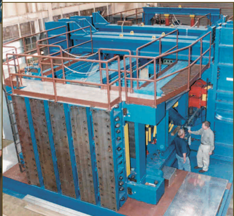
Below: The Grillage Test Facility is used to evaluate the initial ultimate strength and modes of failure as well as post-failure residual strength of full-scale cross-stiffened ship hull plating. Photo by Dr. David Kihl, NSWC Carderock Division.
