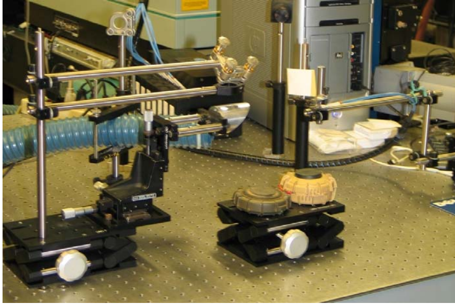
Figure 1. Photo of custom LIBS setup for land mine identification.
