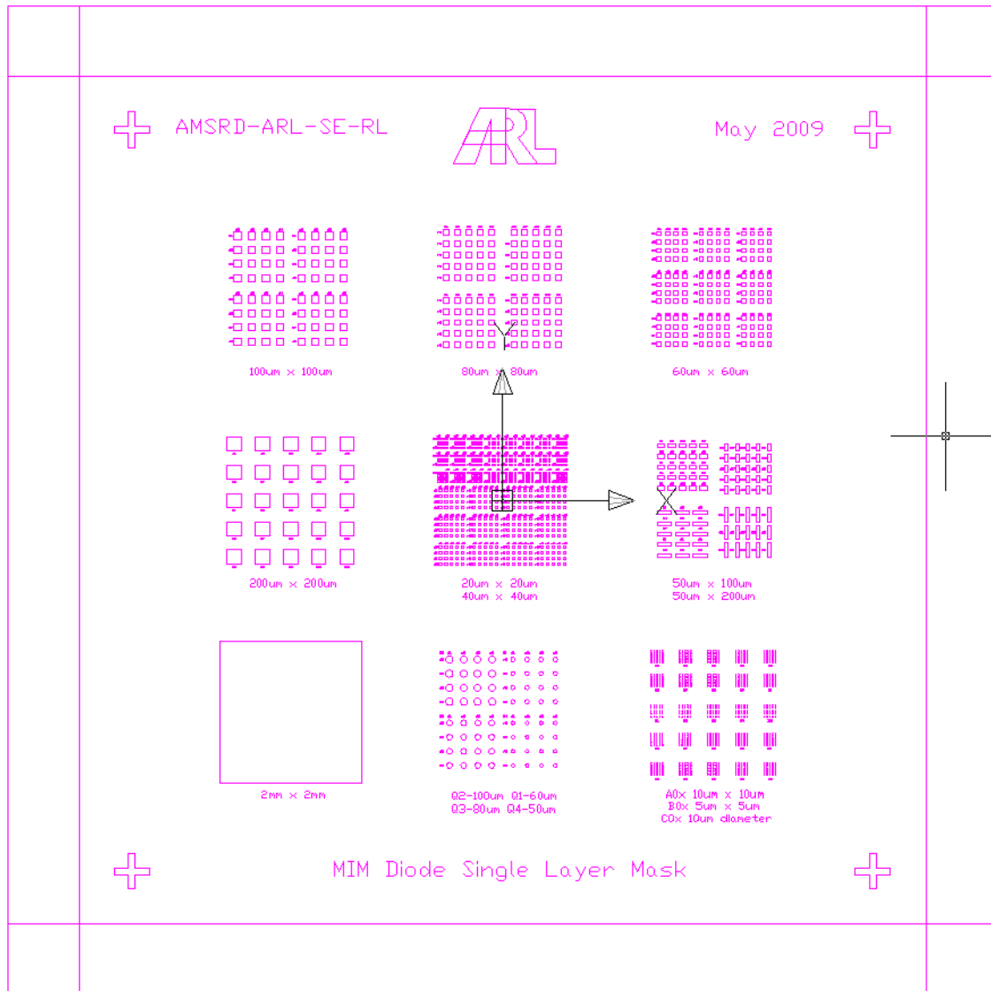
Figure 2. The MIM diode mask provides the patterning for 18 different pillar sizes and geometries ranging from a 2 mm x 2 mm square, to as small as 5 \mu\text{m} x 5 \mu\text{m} squares and 10 \mu\text{m} diameter circles.
