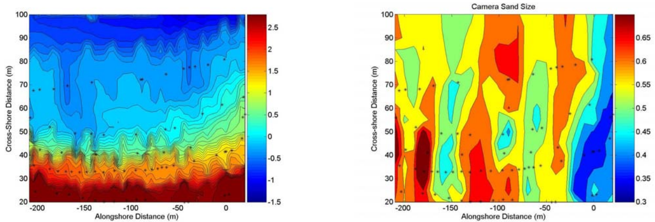
Fig 3. Left panel shows the morphology measured at Sennen (with the color axis in m) using a DGPS system on May 18. The steep forshore slope with beach cusps is visible at the bottom of the panel and the broad intertidal shoal is seen between about 50 and 80 m in the cross shore. The right panel shows grain size estimated with the DIS (with the color axis in mm). The asterisks represent the DIS sample locations. Although the left and right panels are not highly correlated (see text), the grain size variability on this beach is large (0.3- 0.7 mm).
