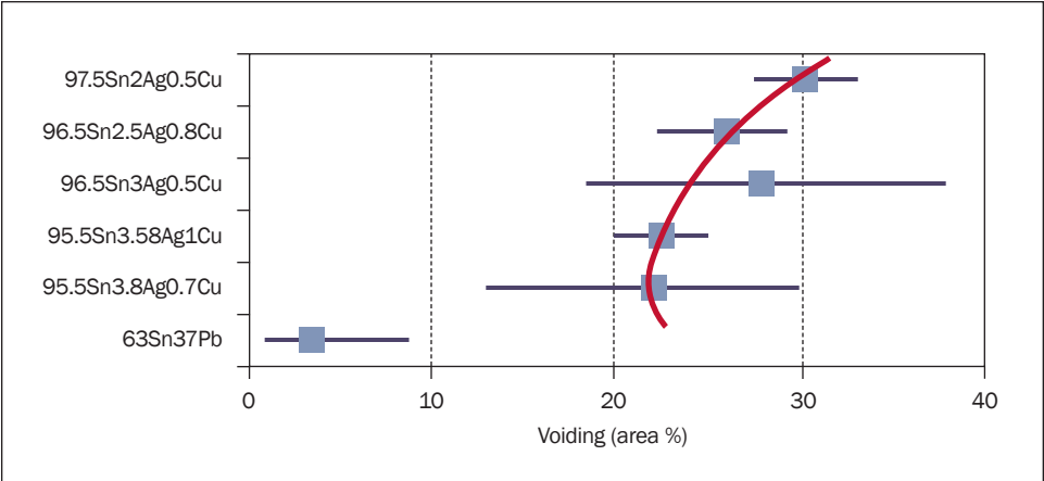
Figure 4.17 Voids in SnPb and Pb-free alloys [6].
