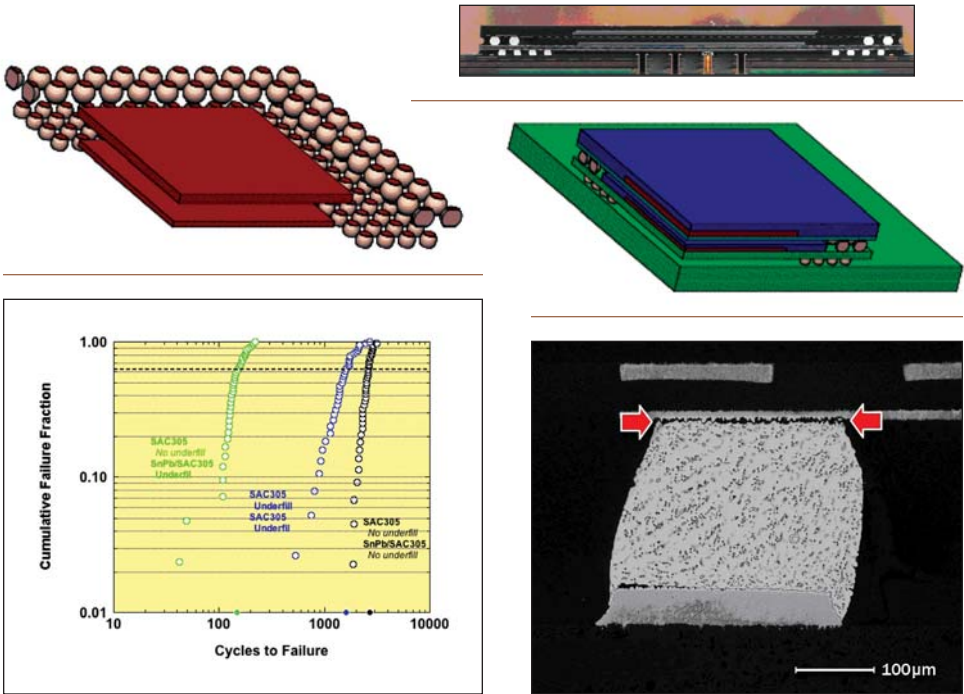
Figure A.6.1 Computational model of package-on-package Pb-free solder joint fatigue.
