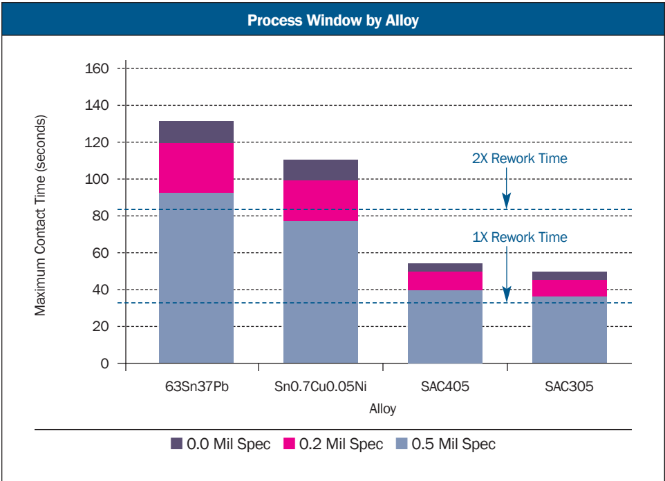
Figure 4.34 The impact of solder alloy selection on the copper dissolution rate during PTH rework.
