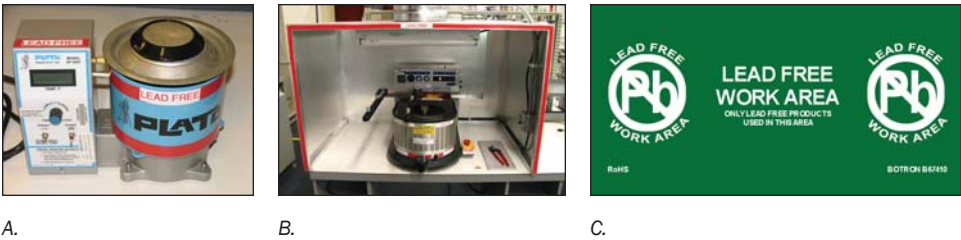
Figure 4.4 Assembly equipment utilizing color marking, designating them as part of a Pb-free solder process only CCA flow. Photos A and B are courtesy of Rockwell Collins; image C is courtesy of Stanley Supply Services.
