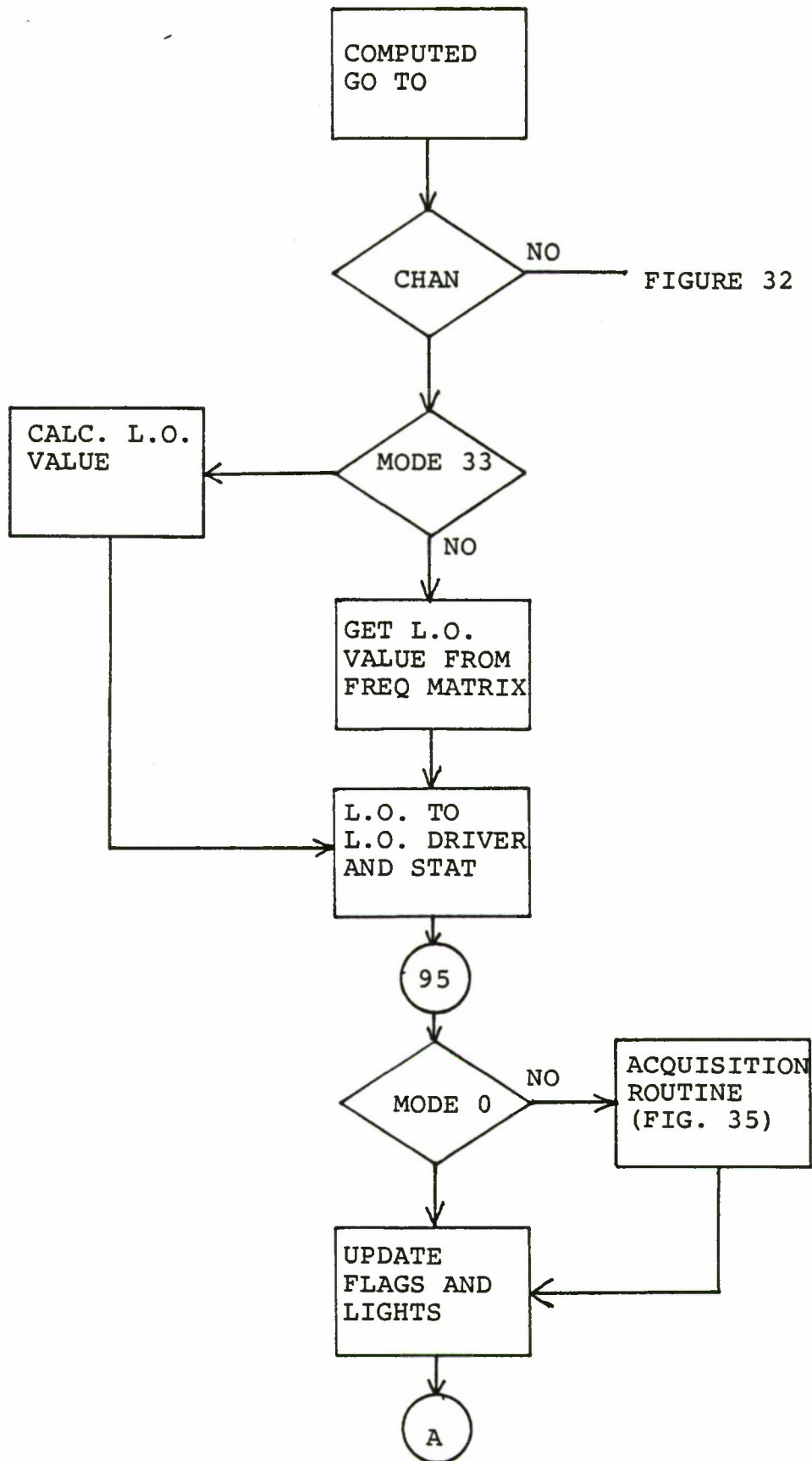
Figure 31 - Enter Button Routine (CHAN)
