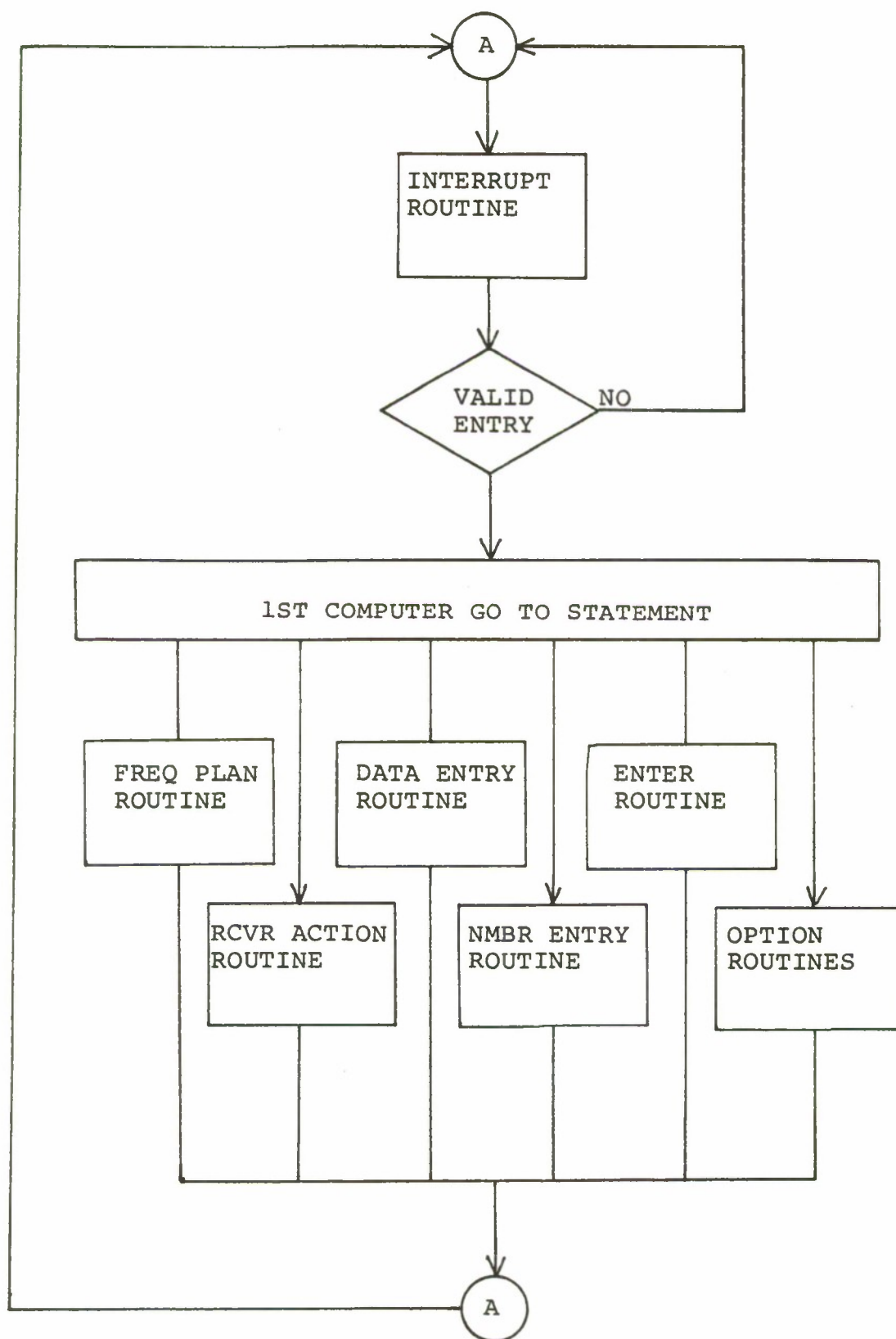
Figure 26 - C2 Operating Program Flowchart
