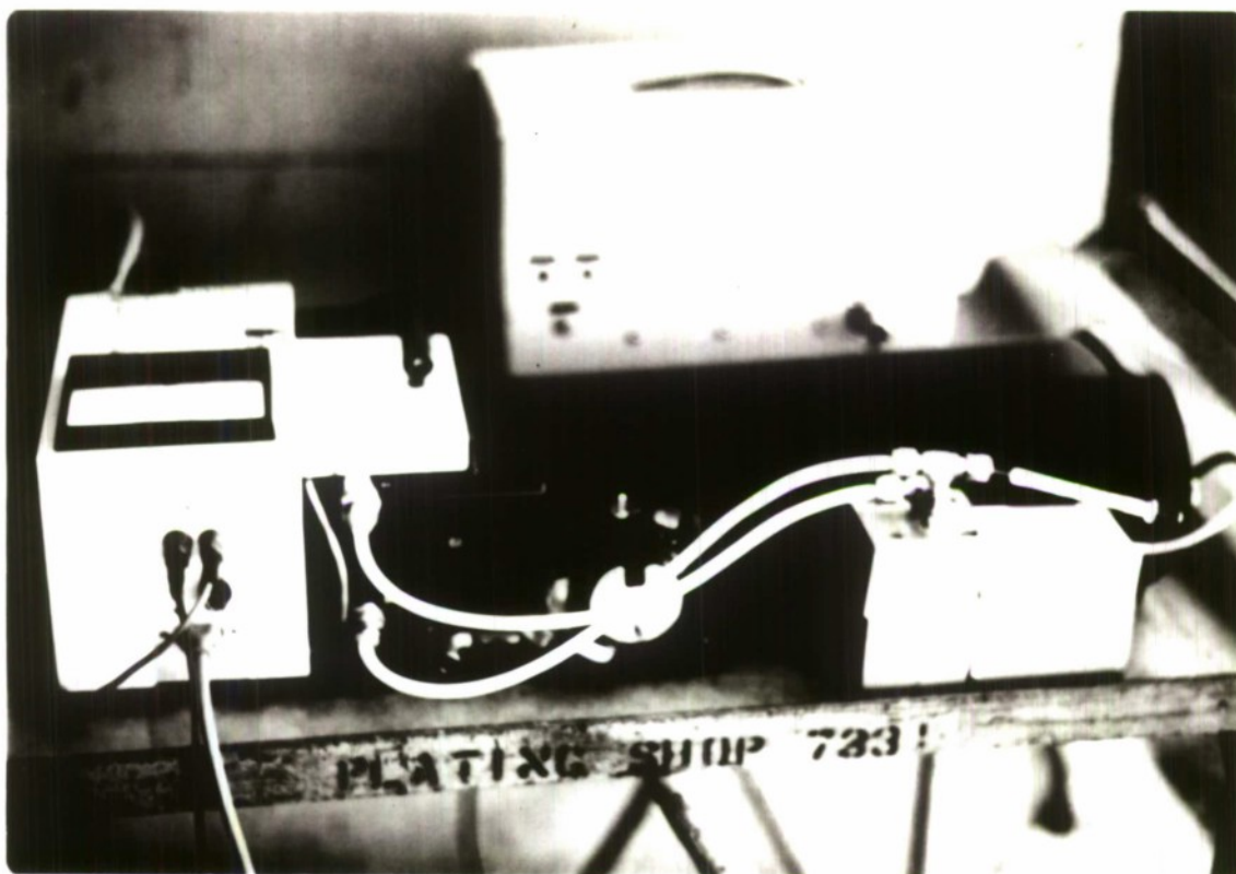
1 (A) MIRAN-1 CALIBRATE MODE INCLUDING INJECTION SYRINGE. ELECTROPLATE SHOP.
