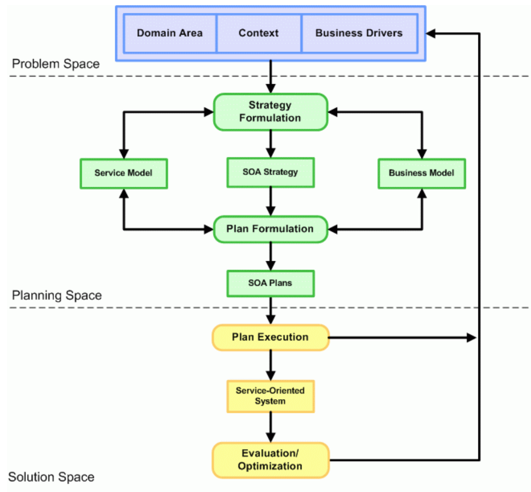
Figure 2: Flow Diagram of the Expanded View of the SOA Problem Space and Solution Space
