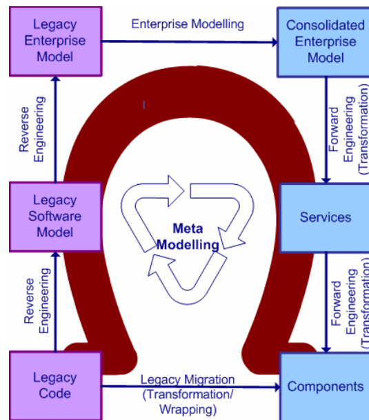
Figure 8: SOA Migration Horseshoe [Winter 2007]
