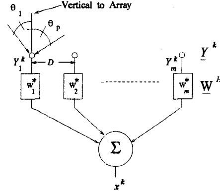
Figure 1: Beamsummer Model.
