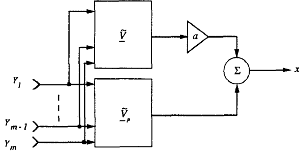
Figure 2: DOA-optimal Beamsummer Block Diagram.
