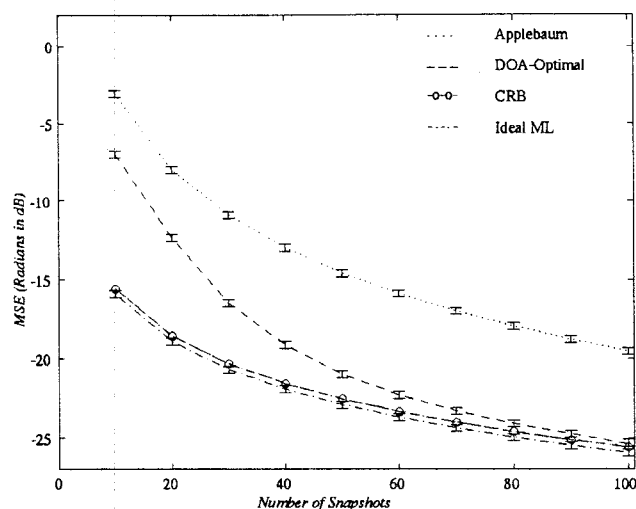
Figure 5: MSE In DOA Estimates: Simulation I.
