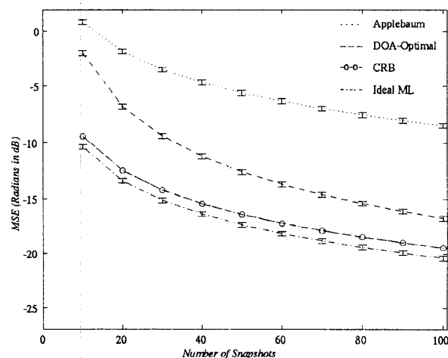
Figure 6: MSE In DOA Estimates: Simulation II.
