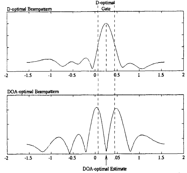
Figure 3: DOA Estimation via Gated Null Picking for a Signal Arriving at \theta = .25 Radians.
