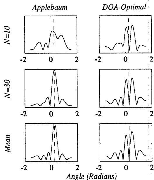
Figure 4: Typical Beampatterns for a Single Realization.
