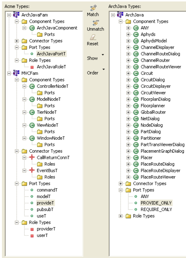
Figure 5.13: AphydsAJ: matching types between Acme (left) and ArchJava (right).
