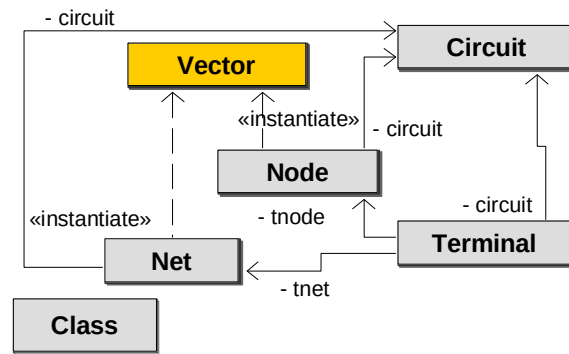
Figure 1.2: Aphyds: partial class diagram focusing on the class Circuit and related classes.
