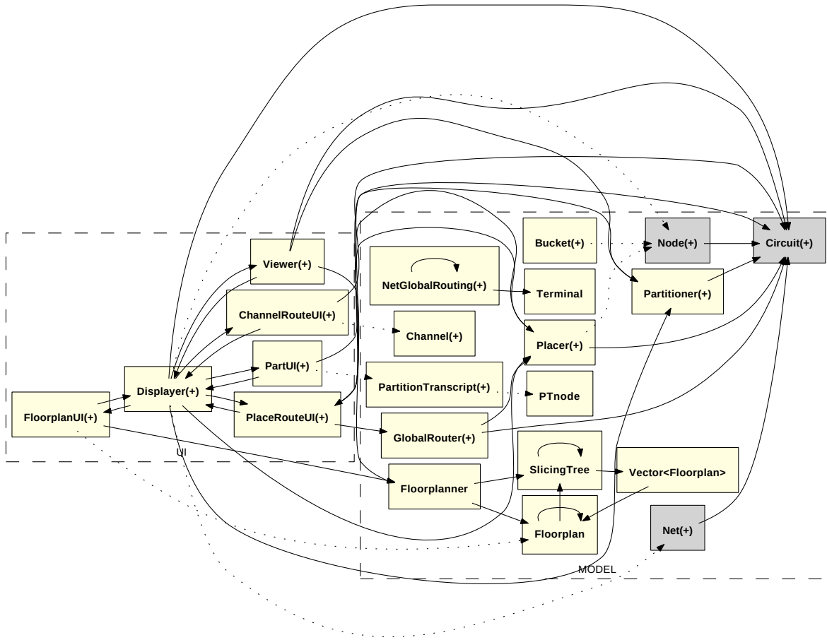
Figure 7.9: Aphyds: OOG using private domains and many peer objects.
