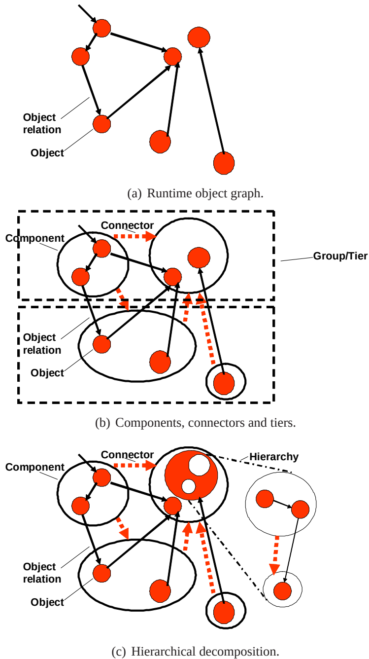
Figure 1.4: Architectural abstraction.
