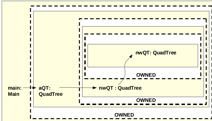
Figure 2.28: QuadTree OOG.
