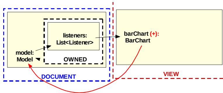
(b) Lifted edge between objects barChart and model.
