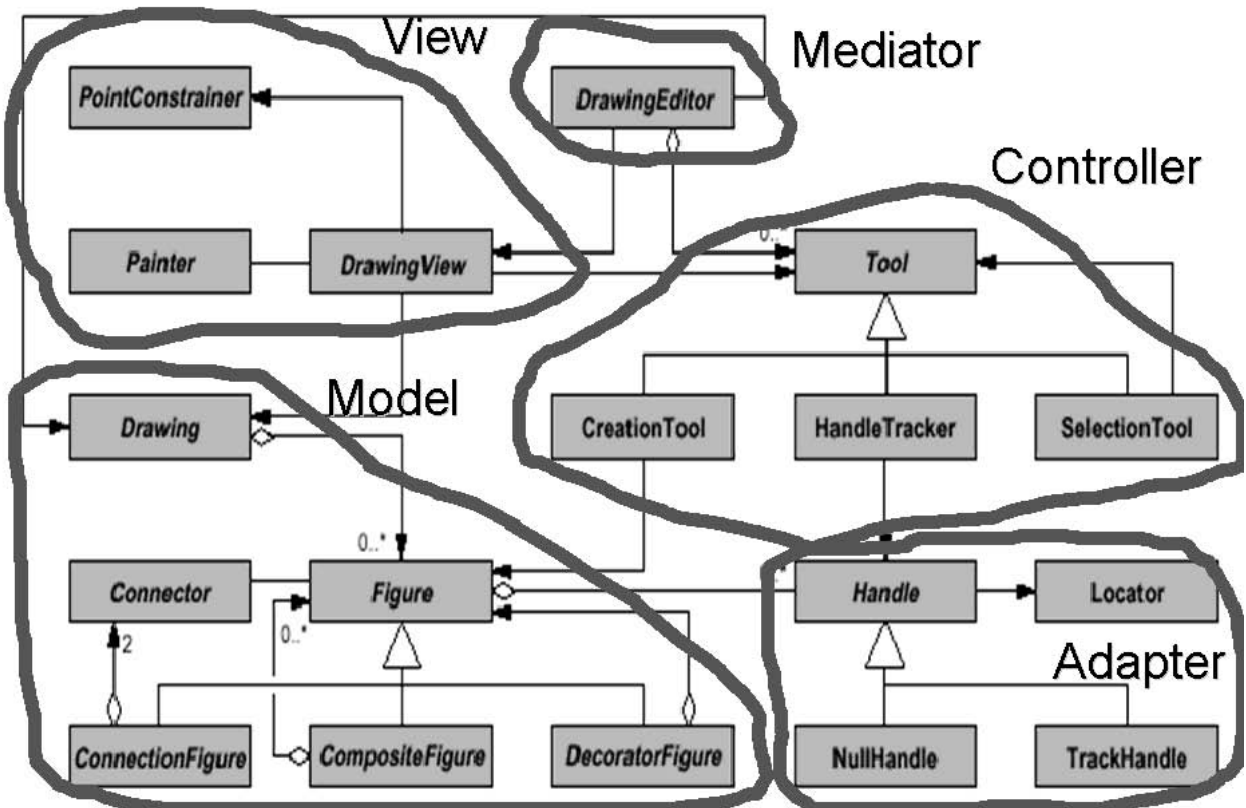
Figure 4.12: JHotDraw: alternative top-level domains. Source: (Christensen 2004).
