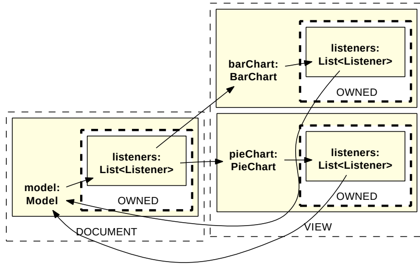
(a) Hierarchical runtime architecture.
