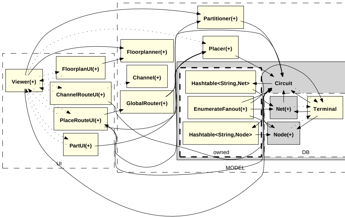
Figure 7.12: Aphyds: refined OOG after defining public domains.
