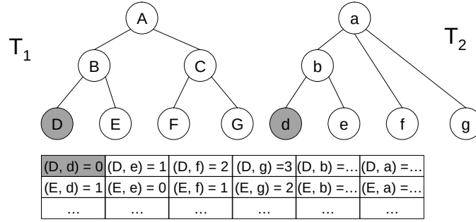
Figure 5.2: \text{COST}(D, d) = cost of editing label of D to d , i.e., the measure of similarity between the labels, in this case 0.
