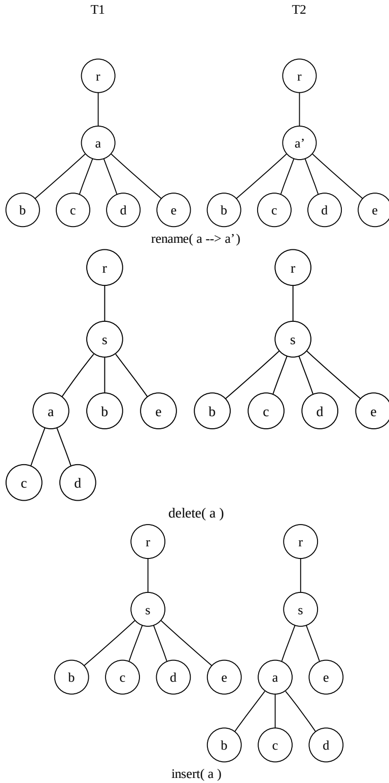
Figure 5.1: Tree edit operations.
