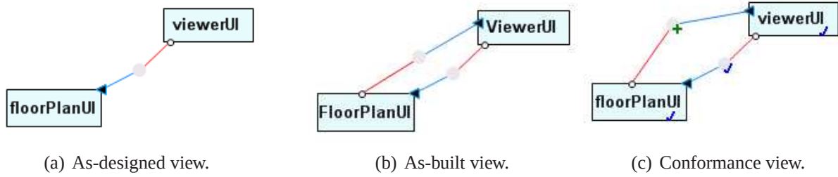
Figure 6.6: Displaying a convergence and a divergence.
