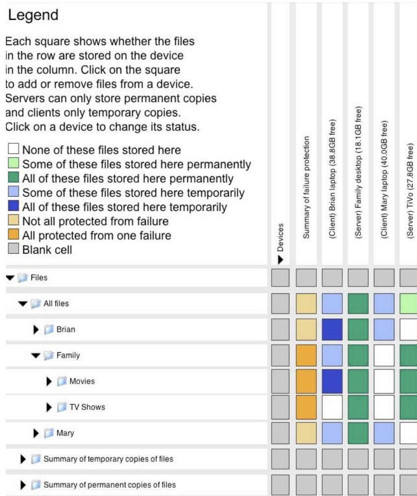
Figure 8.2. Volumes and caching interface. A screen shot of the volume manager GUI. On the left are files, grouped using traditional files-and-folders. Across the top are devices. Each square shows whether the files in the row are stored on the device in the column and whether the copy is temporary or permanent.
