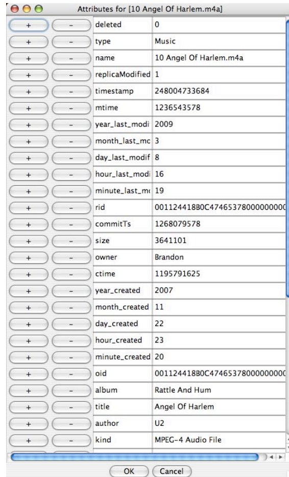
Figure 7.5. Pchatr interface. This figure shows the pchatr interface for manipulating file metdata.
