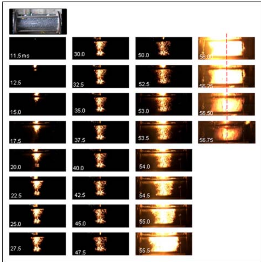
Figure 6. Flamespreading in the 76-cm simulator.
