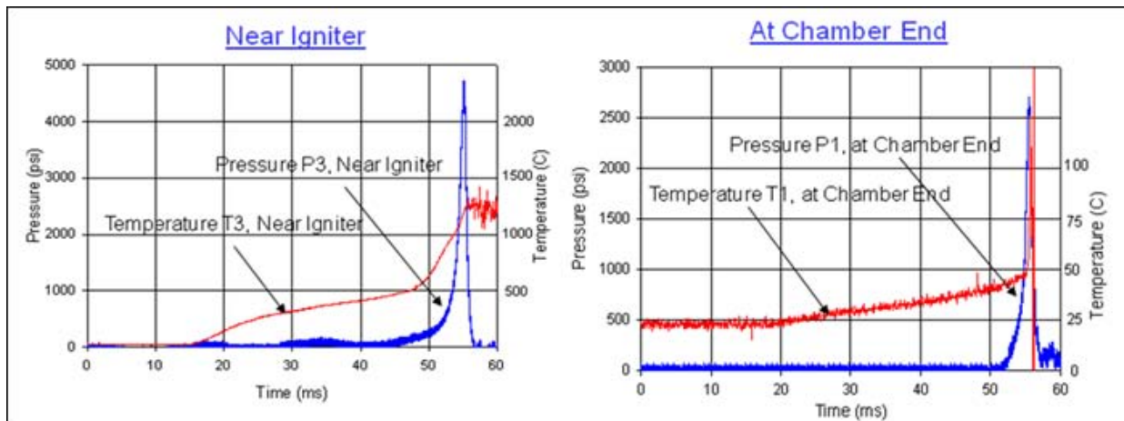
Figure 9. Pressure-time and temperature-time in the 76-cm simulator.
