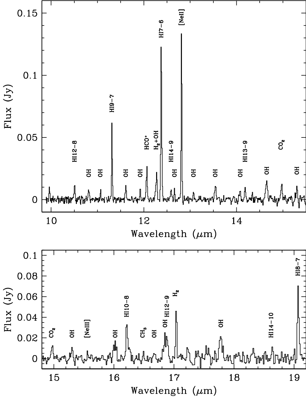
Fig. 2.— Average of the SH1 and SH2 spectra of TW Hya from which a polynomial fit to the continuum has been subtracted. Emission features of atomic lines (HI, [NeII], and possibly [NeIII]) and molecules (H 2 , OH, CO 2 , HCO + , and possibly CH 3 ) are detected. The [NeIII] and CH 3 features are clearer in the SH2 and SH1 spectra, respectively (see Figure 3).
