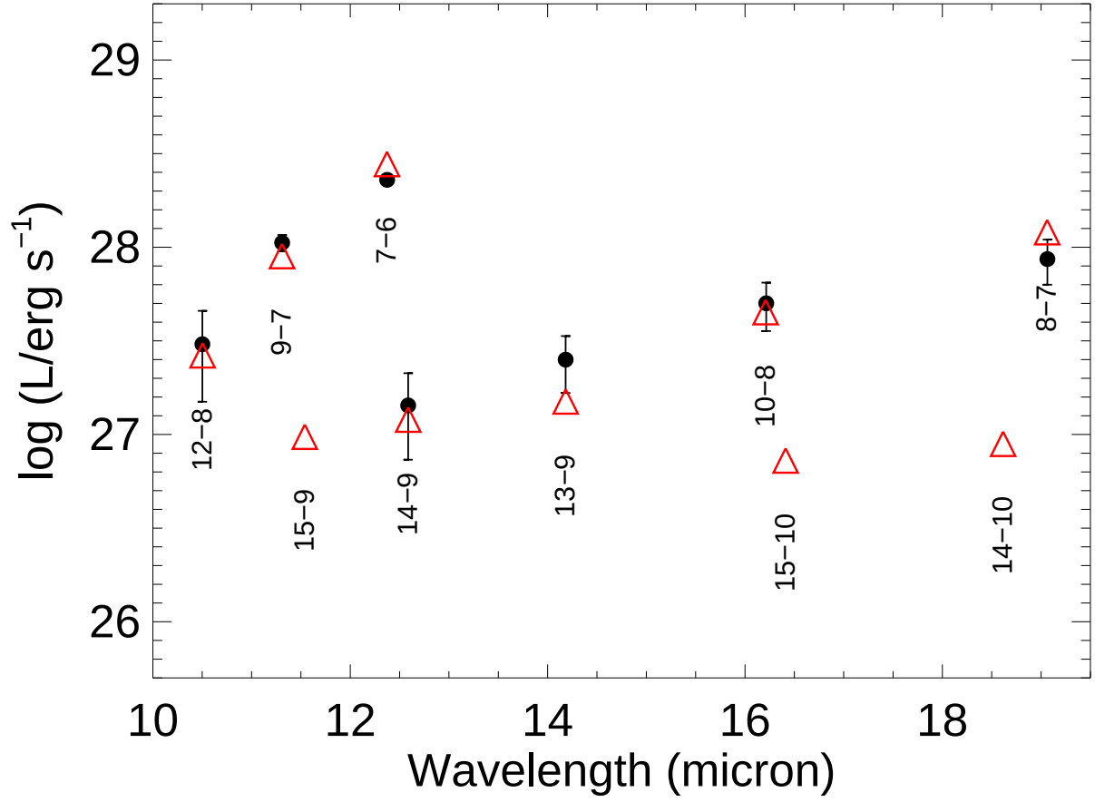
Fig. 6.— HI line luminosities from the SH1 spectrum (dots with error bars) compared with relative fluxes from case B recombination (triangles). The HI 15-9, HI 15-10, and HI 14-10 lines are not detected, consistent with their low anticipated fluxes.
