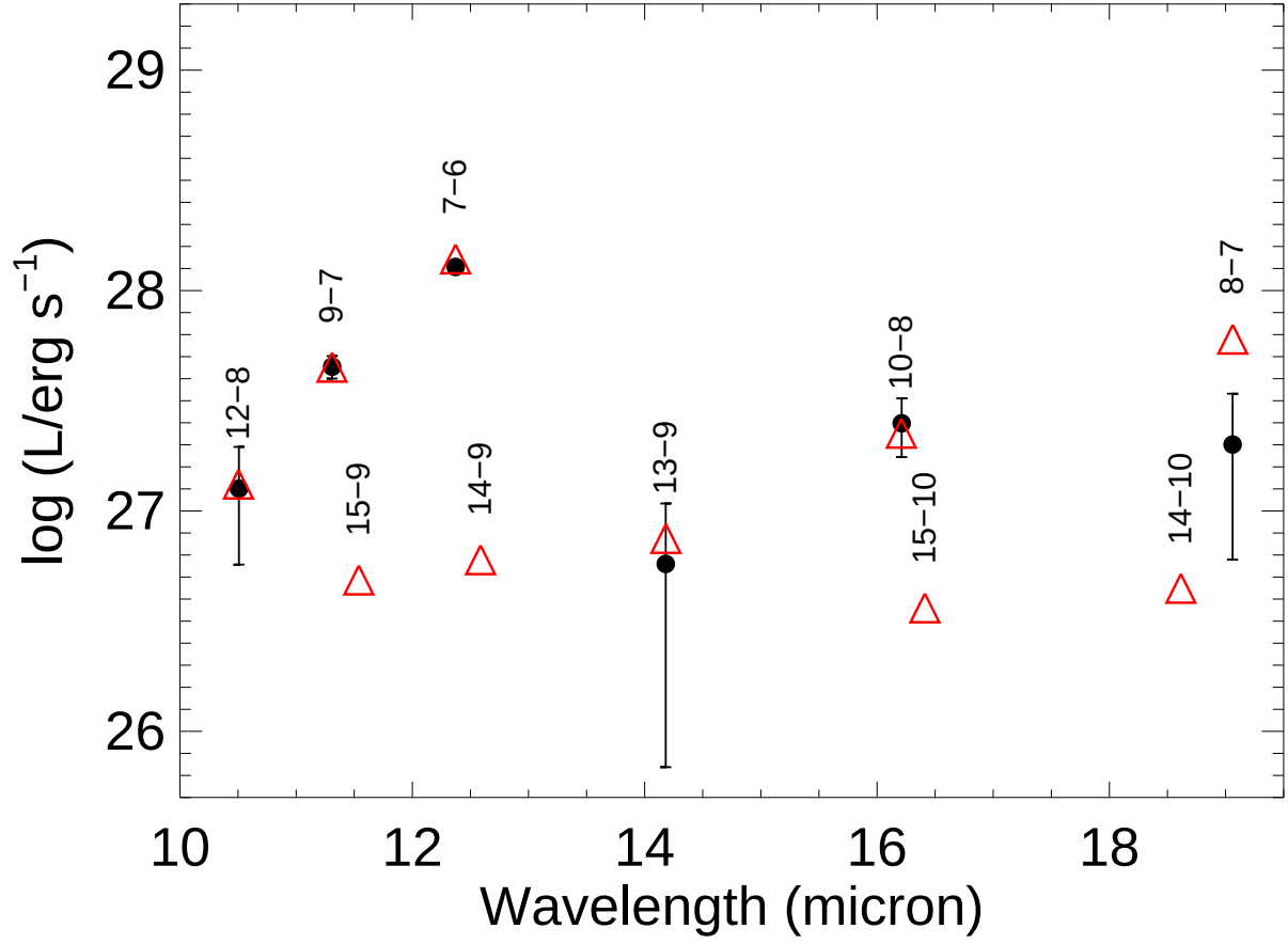
Fig. 7.— HI line luminosities from the SH2 spectrum (dots with error bars) compared with relative fluxes from case B recombination (triangles). The HI 8-7 line is weaker at this epoch and not in as good agreement with the case B relative fluxes. The HI 15-9, HI 14-9, HI 15-10, and HI 14-10 lines are not detected, consistent with their low anticipated fluxes.
