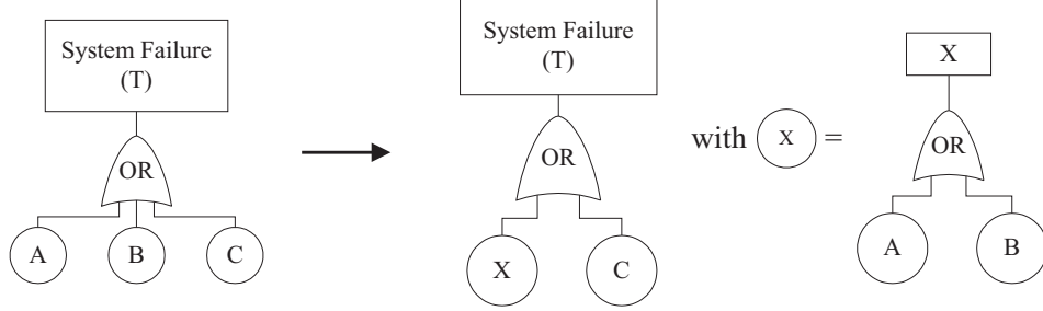
Figure 5: A-B-X Transformation
