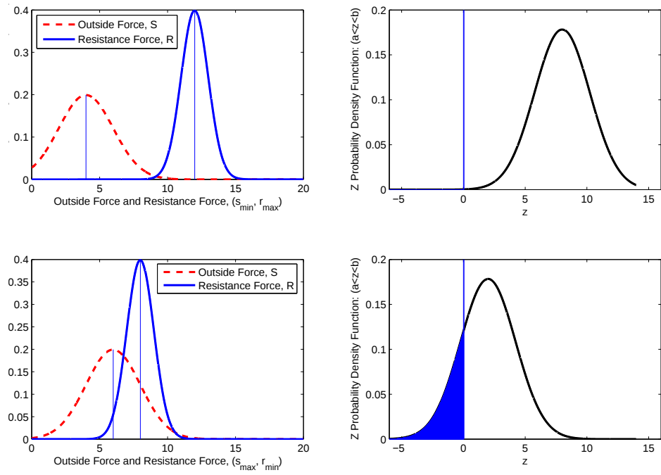
Figure 29: Distributions for S , R , and Z for Best (top) and Worst (bottom) Cases
