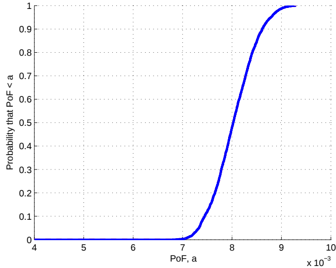
Figure 14: CDF Plot for Pitch Control PoF – Monte Carlo Method
