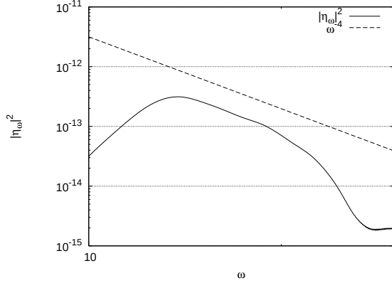
FIG. 3: The time-averaged spectrum of a point on the surface n_\omega = \langle |\eta_\omega|^2 \rangle in the double logarithmic scale. The tail of the distribution fits to the Zakharov-Filonenko spectrum \omega^{-4} .
