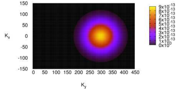
FIG. 1: Initial spectrum |a_{\vec{k}}|^2 . t = 0 .
