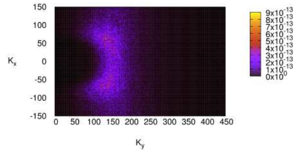
FIG. 2: Final spectrum |a_{\vec{k}}|^2 . t \simeq 2809T_0 .
