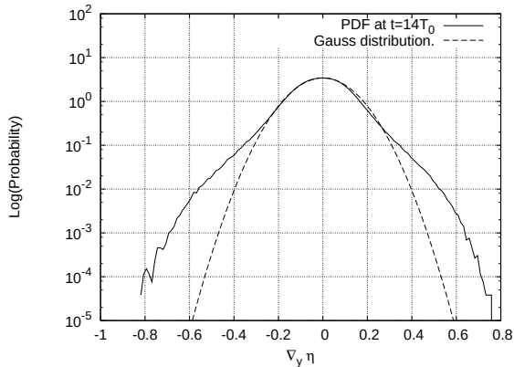
FIG. 4: PDF for (\nabla\eta)_y at the moment of the maximum surface roughness. t \simeq 14T_0 .
