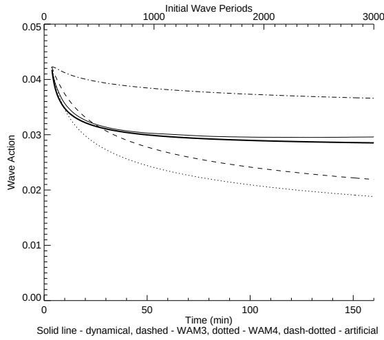
FIG. 5: Total wave action as a function of time. The solid line corresponds to the dynamical equations, the dashed-dotted line — to the kinetic equation with artificial viscosity, the dashed line — to the kinetic equation with the WAM3 damping term, the dotted line — to the kinetic equation with the WAM4 damping term, and the thick solid line — to the kinetic equation with the new damping term,
