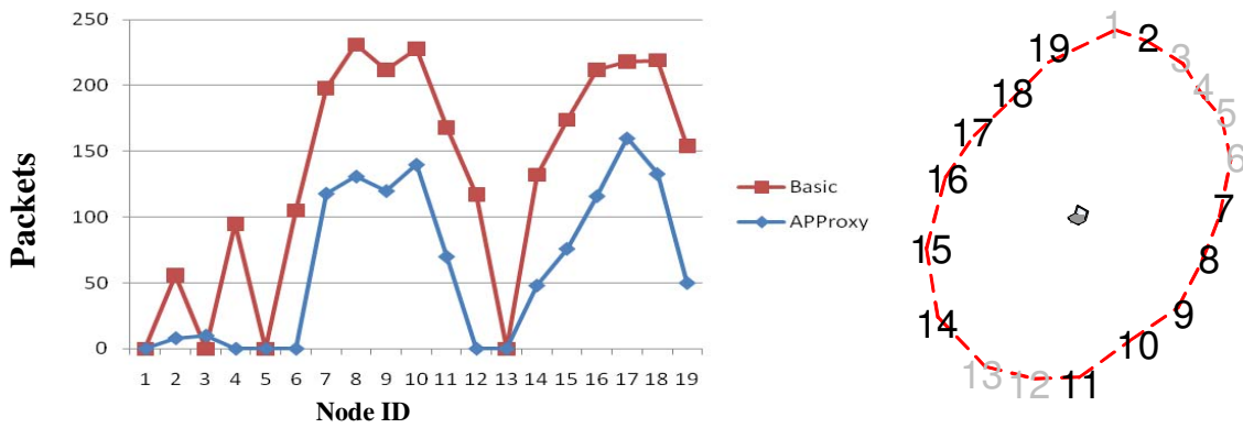
Figure 4-20. Line graph of packet reception between Basic and APProxy patterns with Shadowing model
