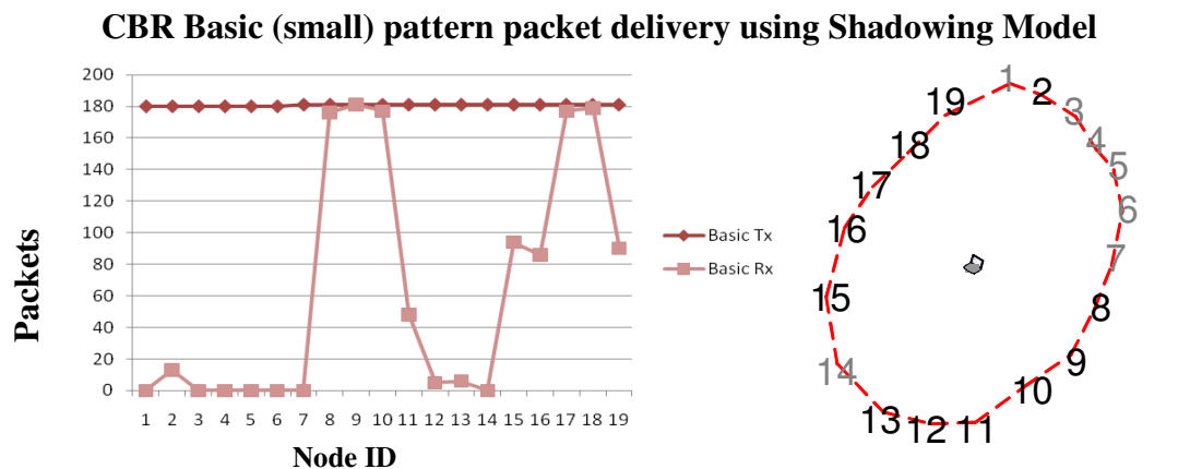
Figure 4-22. Line Graph of packet delivery using the Shadowing Circular shaped propagation pattern
