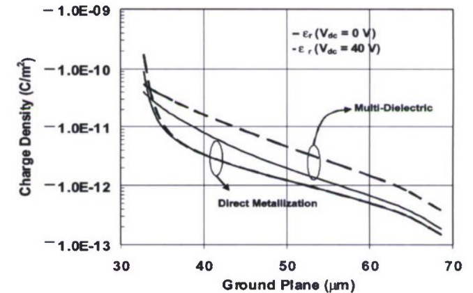
Fig. 8. Charge distributions on the ground-plane conductor for both biased and unbiased cases comparing the multidielectric and the direct metallization cases. Taking symmetry into account (see Fig. 1), only one side of the ground plane (from x = 32.78 to x = 69 \mu\text{m} ) is illustrated.
