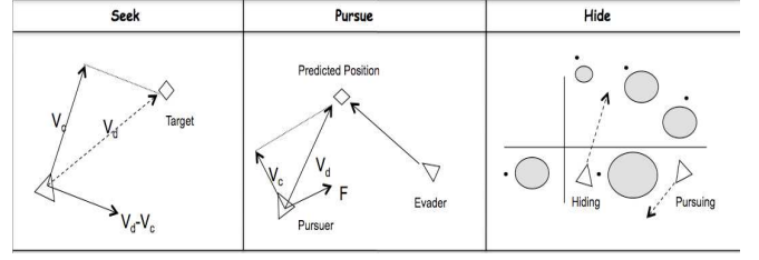
Fig. 3. Individual Steering Forces
