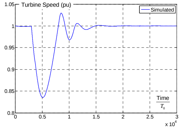
FIGURE 4. Generator speed for CHIL test (normalized scales)
