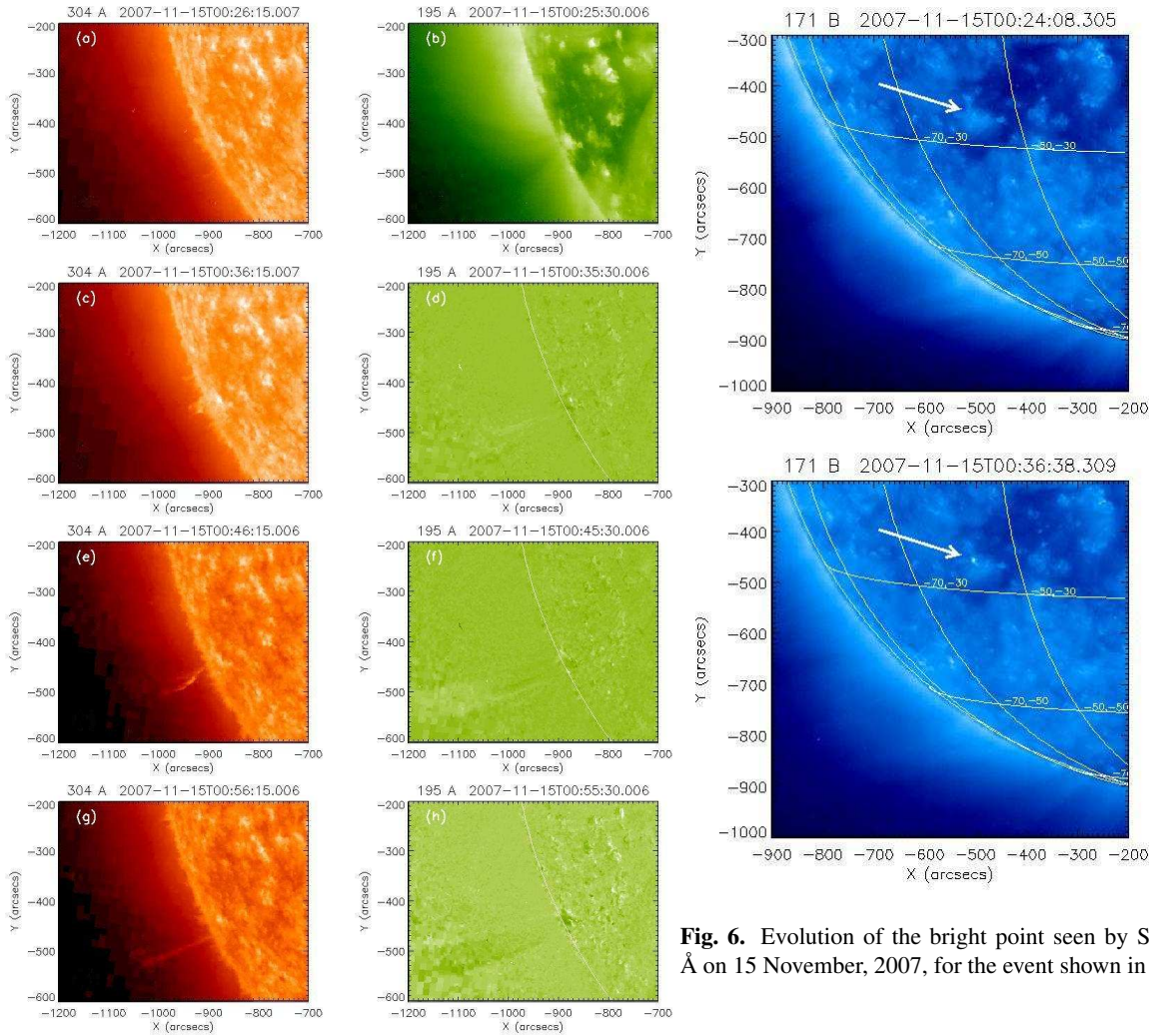
Fig. 5. Evolution of the jet seen by STEREO A at 304 Å and 195 Å on 15 November, 2007. For better visibility, there 195 Å images are shown as difference images.
